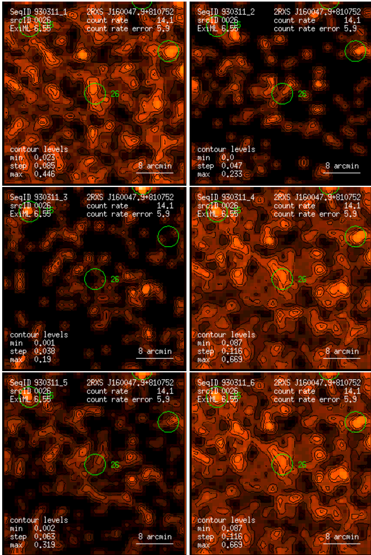
Figure 26: RASS 930311: detection 0026: band rate images, Gaussian filter: (1) PSPC channels 11 – 41, (2) 52 – 90, (3) 91 – 201, (4) 11 – 235, (5) 52 – 201, (6) 11 – 201. Broad band rates in counts/ks. Band rate contour levels in counts/ks/arcmin 2 .
