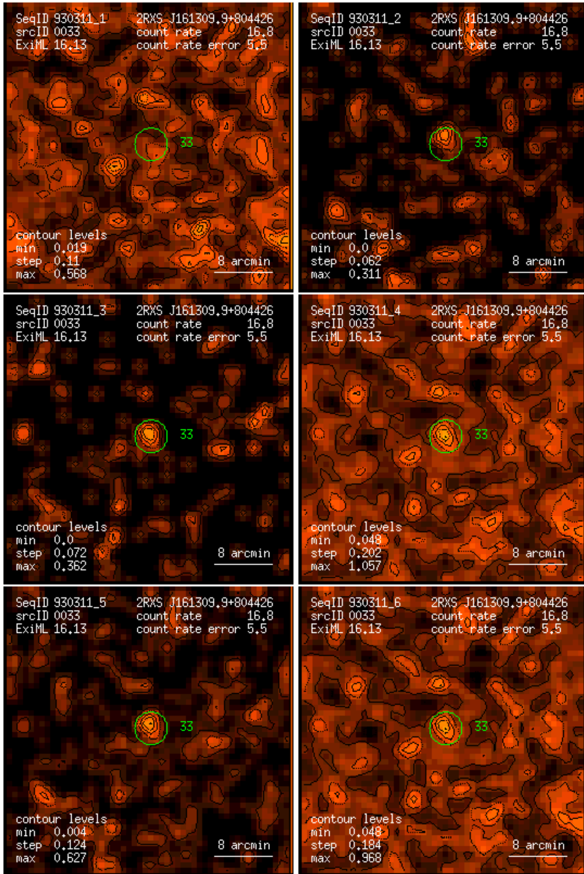
Figure 33: RASS 930311: detection 0033: band rate images, Gaussian filter: (1) PSPC channels 11 – 41, (2) 52 – 90, (3) 91 – 201, (4) 11 – 235, (5) 52 – 201, (6) 11 – 201. Broad band rates in counts/ks. Band rate contour levels in counts/ks/arcmin 2 .
