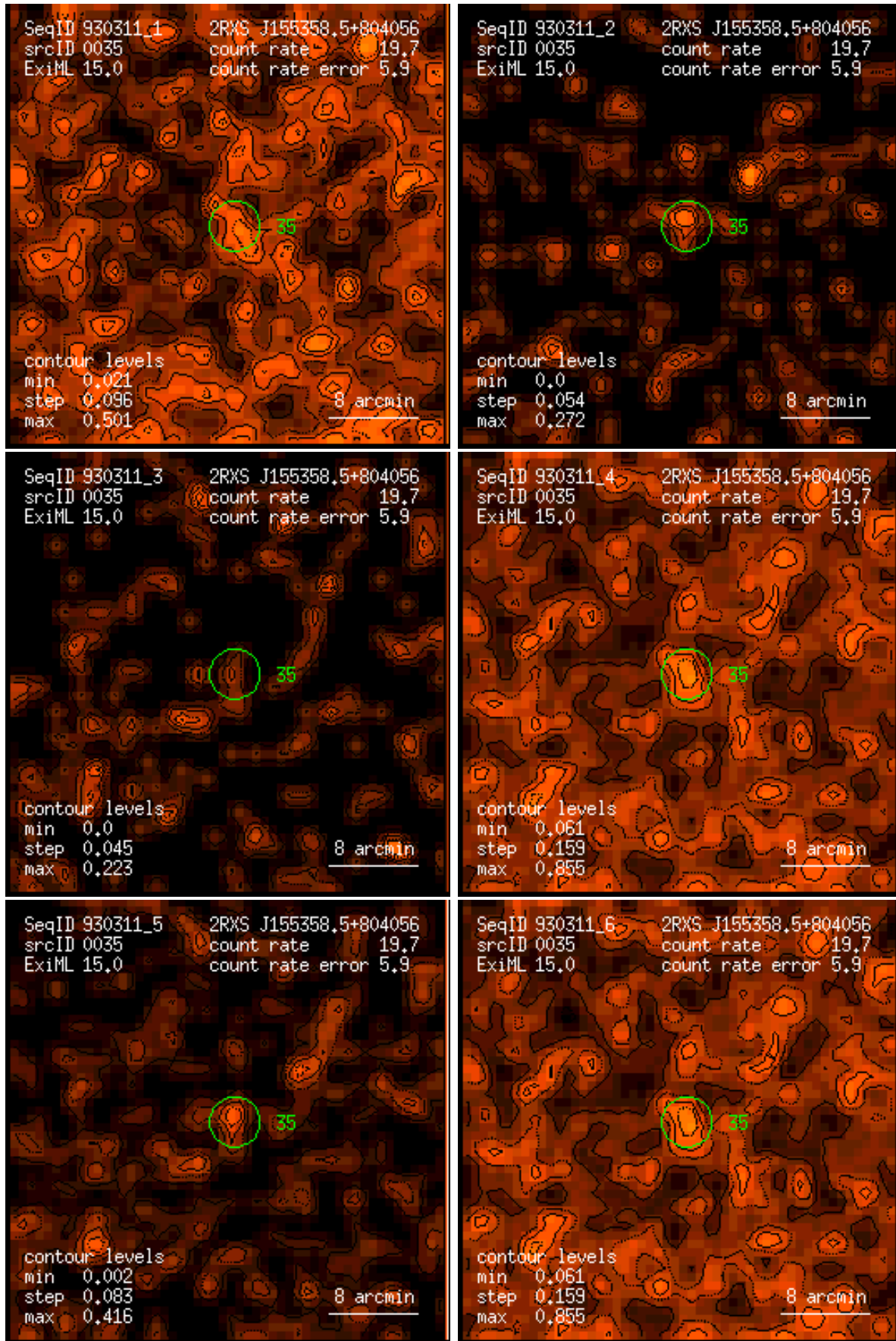
Figure 35: RASS 930311: detection 0035: band rate images, Gaussian filter: (1) PSPC channels 11 – 41, (2) 52 – 90, (3) 91 – 201, (4) 11 – 235, (5) 52 – 201, (6) 11 – 201. Broad band rates in counts/ks. Band rate contour levels in counts/ks/arcmin 2 .
