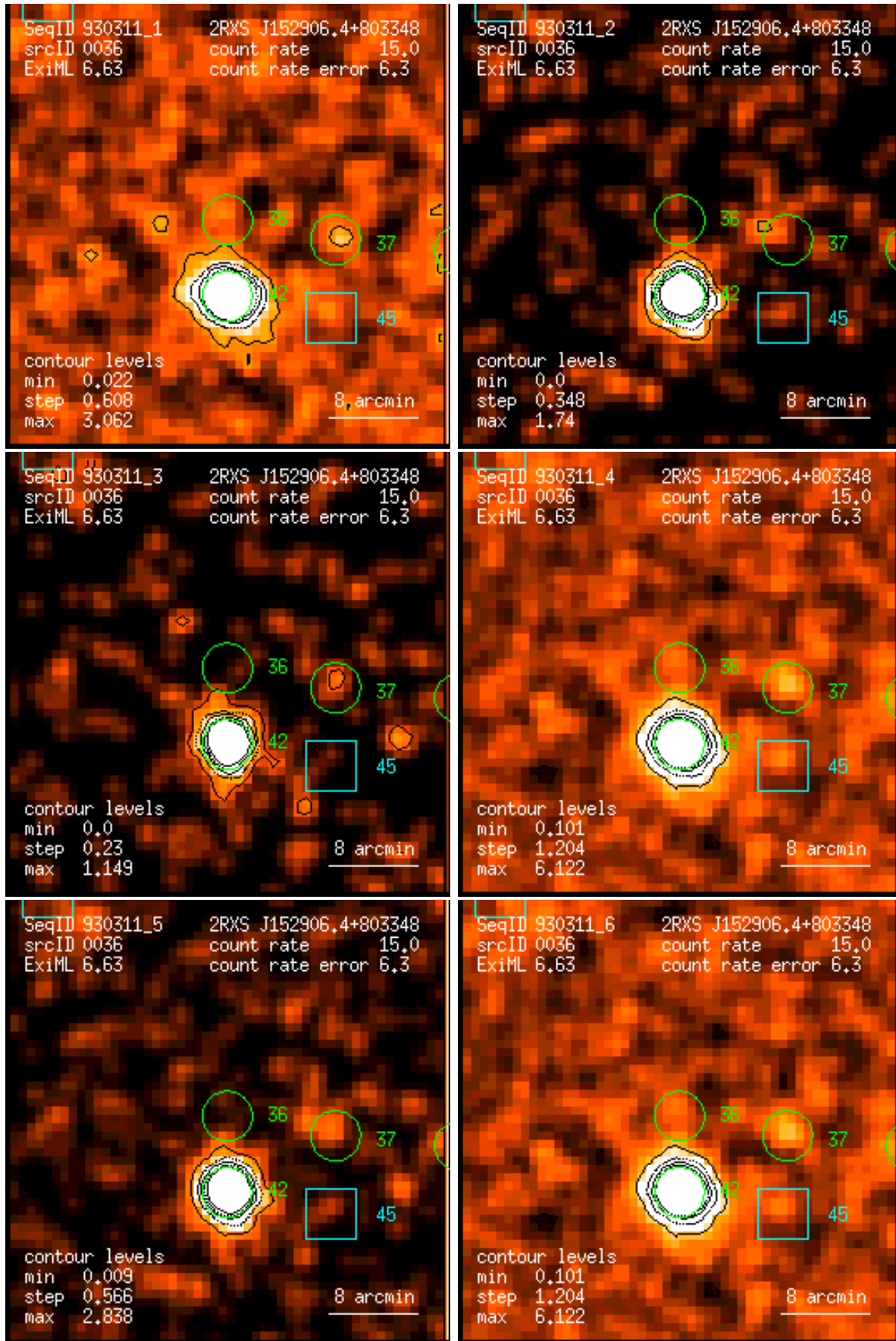
Figure 36: RASS 930311: detection 0036: band rate images, Gaussian filter: (1) PSPC channels 11 – 41, (2) 52 – 90, (3) 91 – 201, (4) 11 – 235, (5) 52 – 201, (6) 11 – 201. Broad band rates in counts/ks. Band rate contour levels in counts/ks/arcmin 2 .
