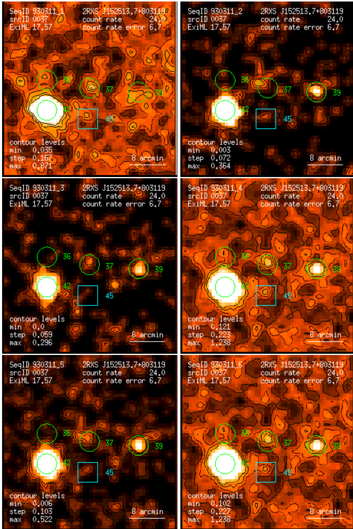
Figure 37: RASS 930311: detection 0037: band rate images, Gaussian filter: (1) PSPC channels 11 – 41, (2) 52 – 90, (3) 91 – 201, (4) 11 – 235, (5) 52 – 201, (6) 11 – 201. Broad band rates in counts/ks. Band rate contour levels in counts/ks/arcmin 2 .
