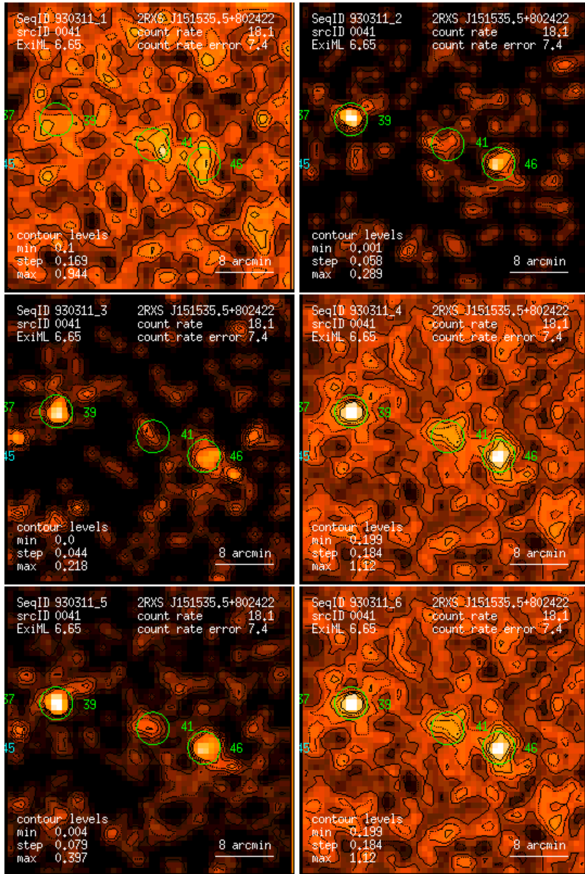
Figure 41: RASS 930311: detection 0041: band rate images, Gaussian filter: (1) PSPC channels 11 – 41, (2) 52 – 90, (3) 91 – 201, (4) 11 – 235, (5) 52 – 201, (6) 11 – 201. Broad band rates in counts/ks. Band rate contour levels in counts/ks/arcmin 2 .
