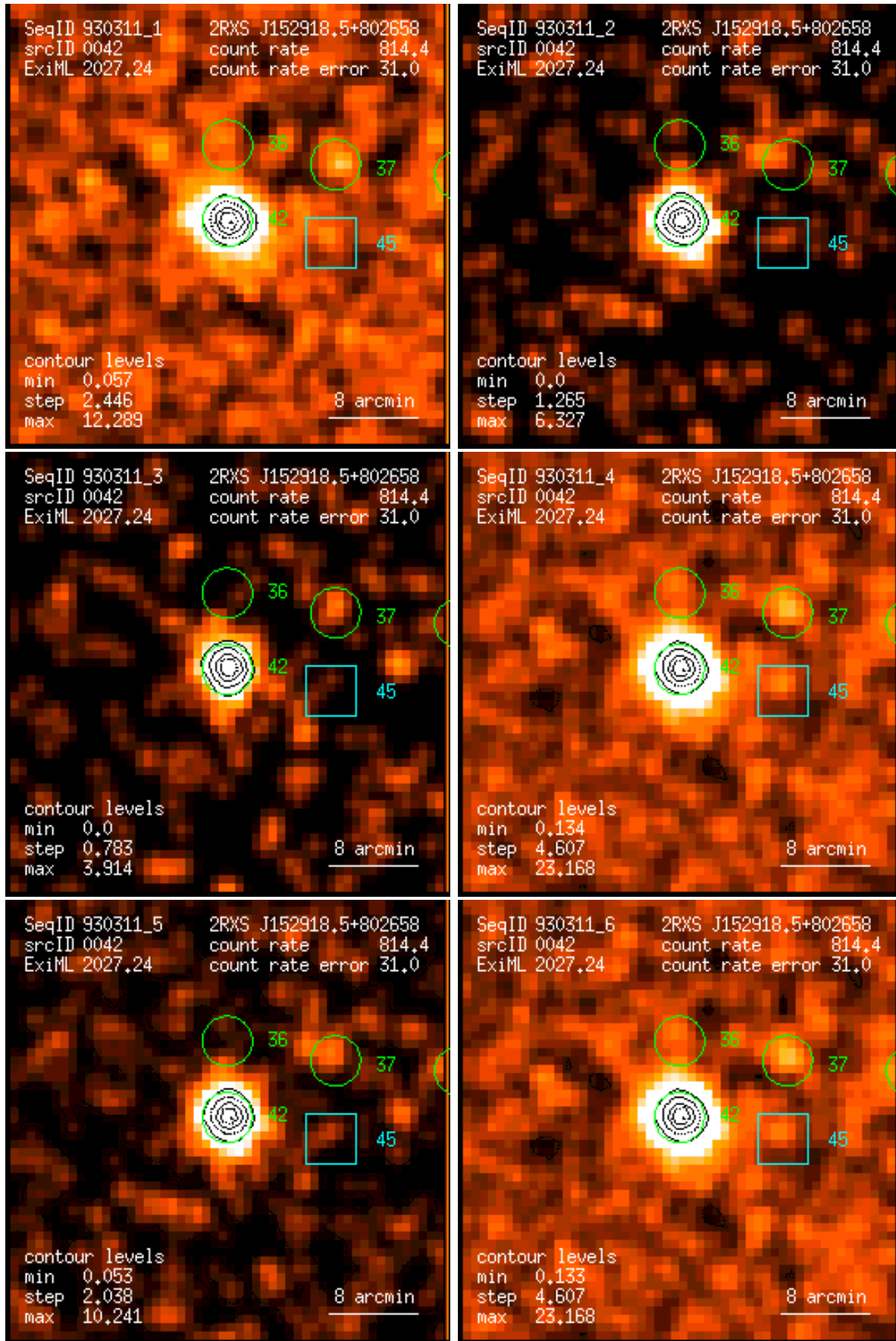
Figure 42: RASS 930311: detection 0042: band rate images, Gaussian filter: (1) PSPC channels 11 – 41, (2) 52 – 90, (3) 91 – 201, (4) 11 – 235, (5) 52 – 201, (6) 11 – 201. Broad band rates in counts/ks. Band rate contour levels in counts/ks/arcmin 2 .
