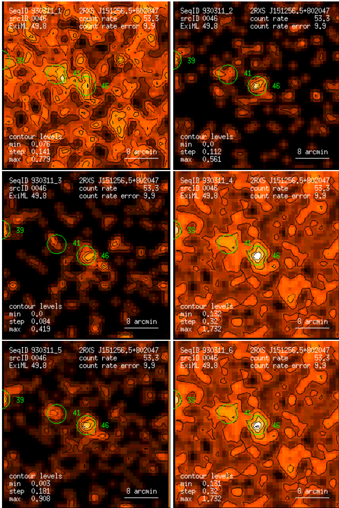
Figure 46: RASS 930311: detection 0046: band rate images, Gaussian filter: (1) PSPC channels 11 – 41, (2) 52 – 90, (3) 91 – 201, (4) 11 – 235, (5) 52 – 201, (6) 11 – 201. Broad band rates in counts/ks. Band rate contour levels in counts/ks/arcmin 2 .
