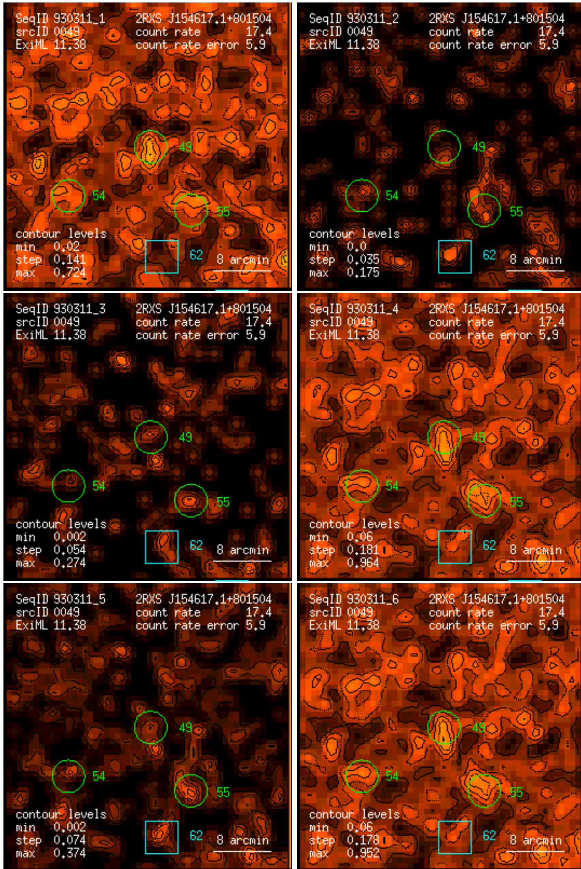
Figure 49: RASS 930311: detection 0049: band rate images, Gaussian filter: (1) PSPC channels 11 – 41, (2) 52 – 90, (3) 91 – 201, (4) 11 – 235, (5) 52 – 201, (6) 11 – 201. Broad band rates in counts/ks. Band rate contour levels in counts/ks/arcmin 2 .
