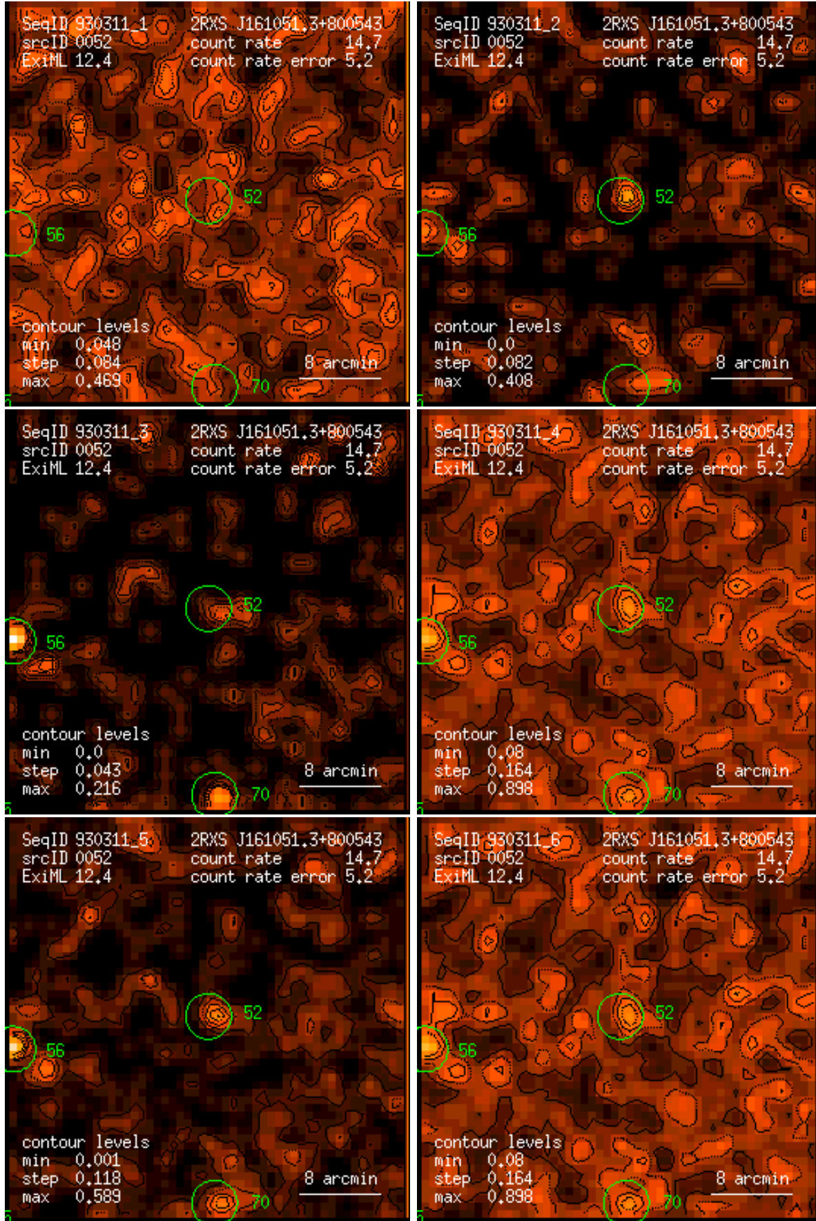
Figure 52: RASS 930311: detection 0052: band rate images, Gaussian filter: (1) PSPC channels 11 – 41, (2) 52 – 90, (3) 91 – 201, (4) 11 – 235, (5) 52 – 201, (6) 11 – 201. Broad band rates in counts/ks. Band rate contour levels in counts/ks/arcmin 2 .
