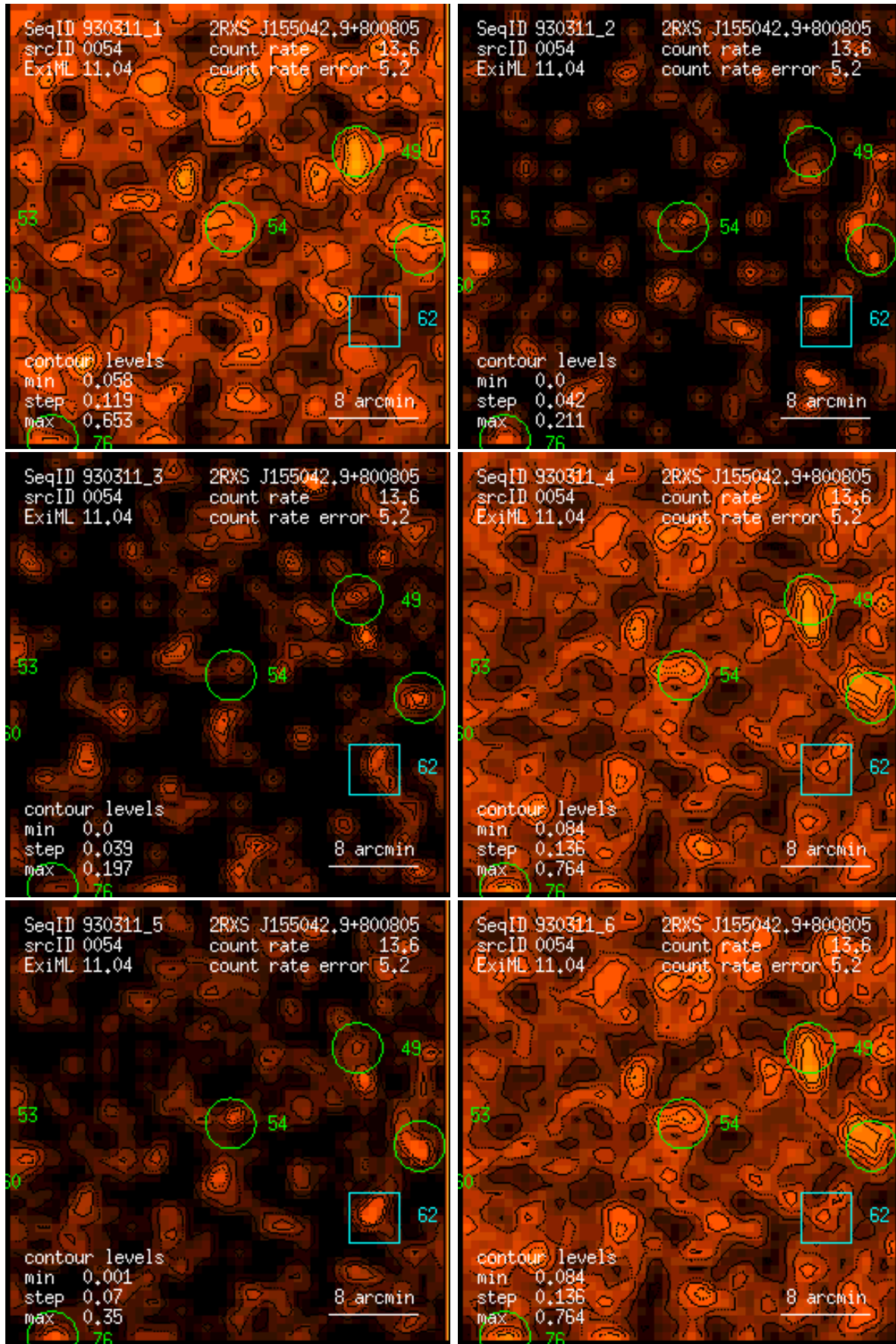
Figure 54: RASS 930311: detection 0054: band rate images, Gaussian filter: (1) PSPC channels 11 – 41, (2) 52 – 90, (3) 91 – 201, (4) 11 – 235, (5) 52 – 201, (6) 11 – 201. Broad band rates in counts/ks. Band rate contour levels in counts/ks/arcmin 2 .
