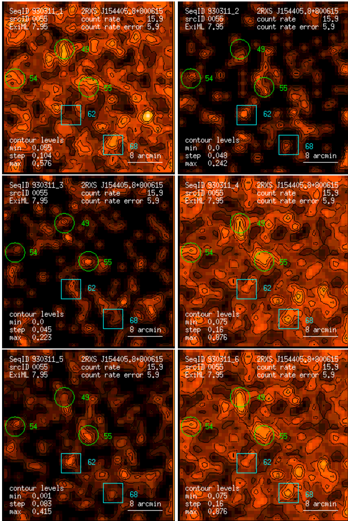
Figure 55: RASS 930311: detection 0055: band rate images, Gaussian filter: (1) PSPC channels 11 – 41, (2) 52 – 90, (3) 91 – 201, (4) 11 – 235, (5) 52 – 201, (6) 11 – 201. Broad band rates in counts/ks. Band rate contour levels in counts/ks/arcmin 2 .
