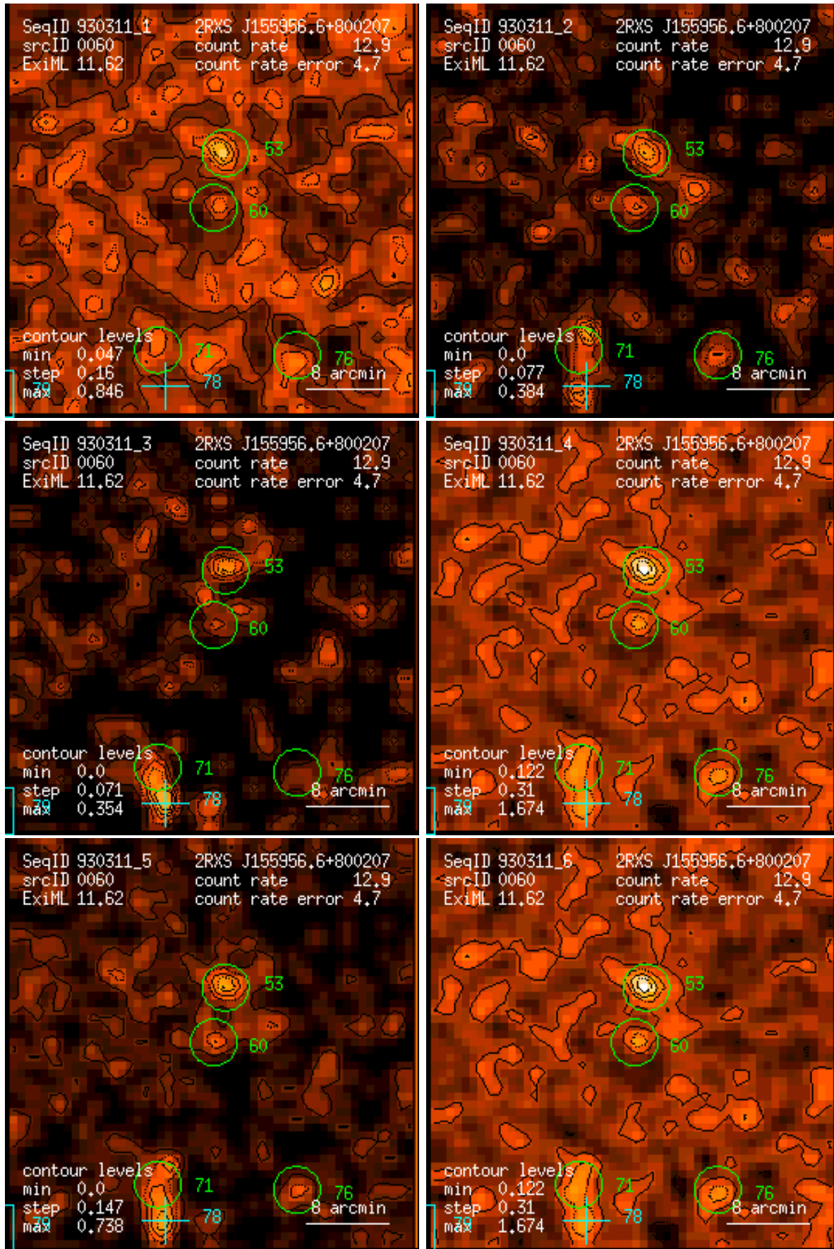
Figure 60: RASS 930311: detection 0060: band rate images, Gaussian filter: (1) PSPC channels 11 – 41, (2) 52 – 90, (3) 91 – 201, (4) 11 – 235, (5) 52 – 201, (6) 11 – 201. Broad band rates in counts/ks. Band rate contour levels in counts/ks/arcmin 2 .
