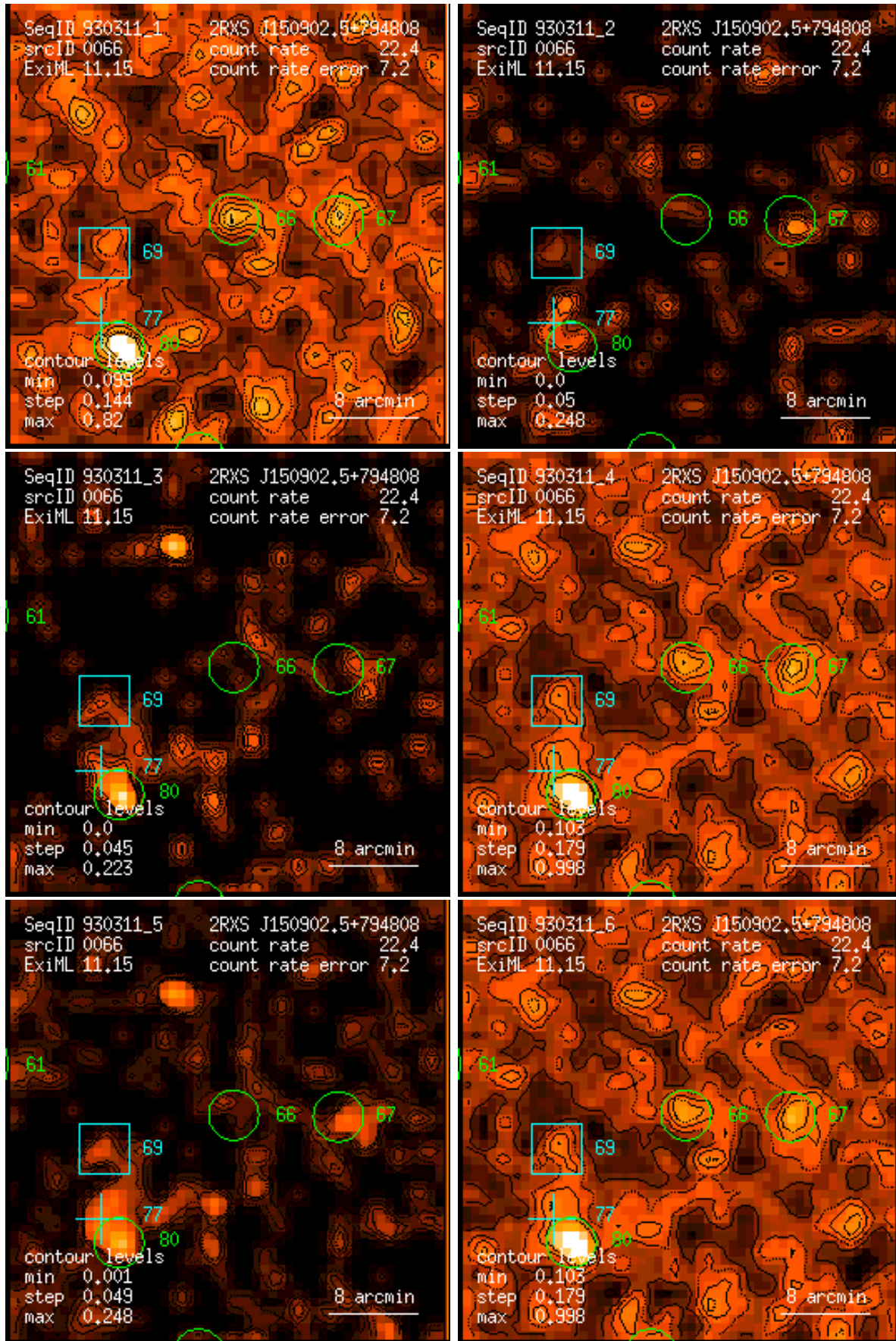
Figure 66: RASS 930311: detection 0066: band rate images, Gaussian filter: (1) PSPC channels 11 – 41, (2) 52 – 90, (3) 91 – 201, (4) 11 – 235, (5) 52 – 201, (6) 11 – 201. Broad band rates in counts/ks. Band rate contour levels in counts/ks/arcmin 2 .
