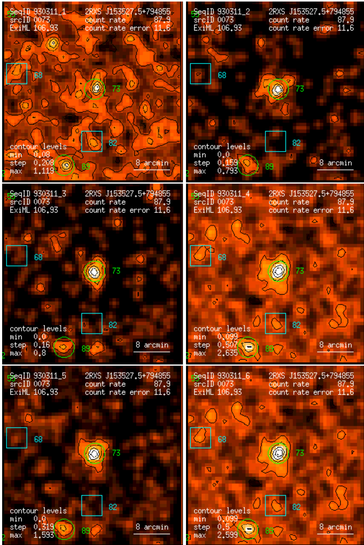
Figure 73: RASS 930311: detection 0073: band rate images, Gaussian filter: (1) PSPC channels 11 – 41, (2) 52 – 90, (3) 91 – 201, (4) 11 – 235, (5) 52 – 201, (6) 11 – 201. Broad band rates in counts/ks. Band rate contour levels in counts/ks/arcmin 2 .
