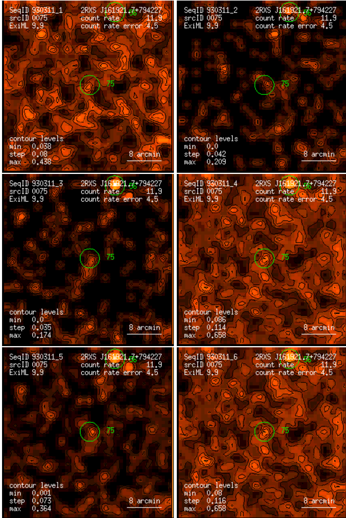
Figure 75: RASS 930311: detection 0075: band rate images, Gaussian filter: (1) PSPC channels 11 – 41, (2) 52 – 90, (3) 91 – 201, (4) 11 – 235, (5) 52 – 201, (6) 11 – 201. Broad band rates in counts/ks. Band rate contour levels in counts/ks/arcmin 2 .
