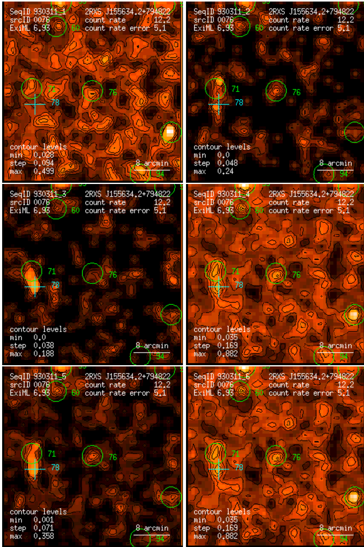
Figure 76: RASS 930311: detection 0076: band rate images, Gaussian filter: (1) PSPC channels 11 – 41, (2) 52 – 90, (3) 91 – 201, (4) 11 – 235, (5) 52 – 201, (6) 11 – 201. Broad band rates in counts/ks. Band rate contour levels in counts/ks/arcmin 2 .
