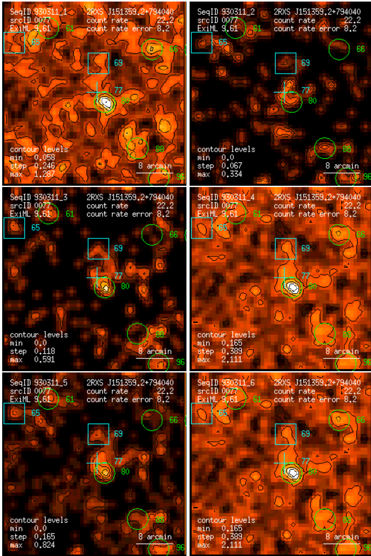
Figure 77: RASS 930311: detection 0077: band rate images, Gaussian filter: (1) PSPC channels 11 – 41, (2) 52 – 90, (3) 91 – 201, (4) 11 – 235, (5) 52 – 201, (6) 11 – 201. Broad band rates in counts/ks. Band rate contour levels in counts/ks/arcmin 2 .
