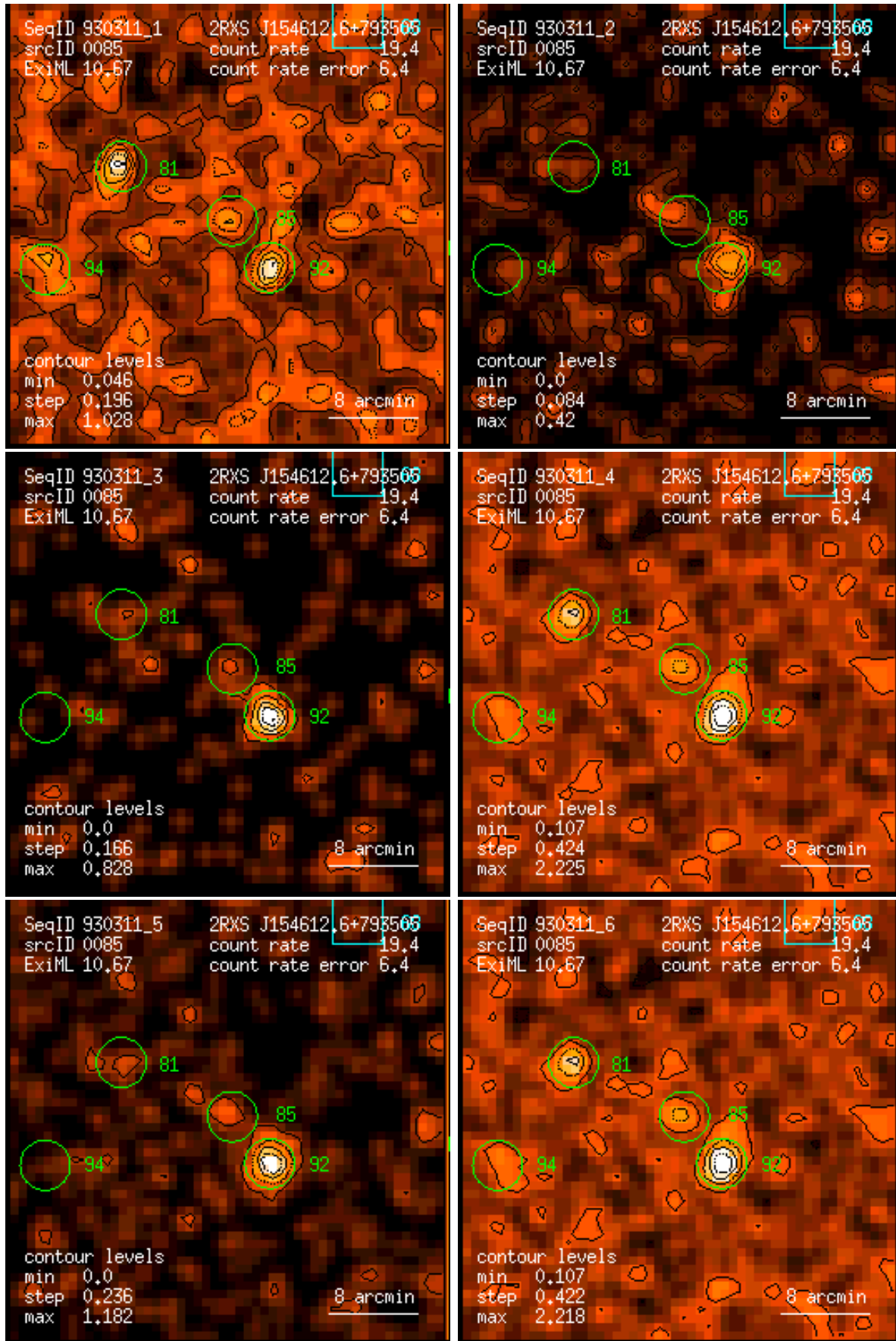
Figure 85: RASS 930311: detection 0085: band rate images, Gaussian filter: (1) PSPC channels 11 – 41, (2) 52 – 90, (3) 91 – 201, (4) 11 – 235, (5) 52 – 201, (6) 11 – 201. Broad band rates in counts/ks. Band rate contour levels in counts/ks/arcmin 2 .
