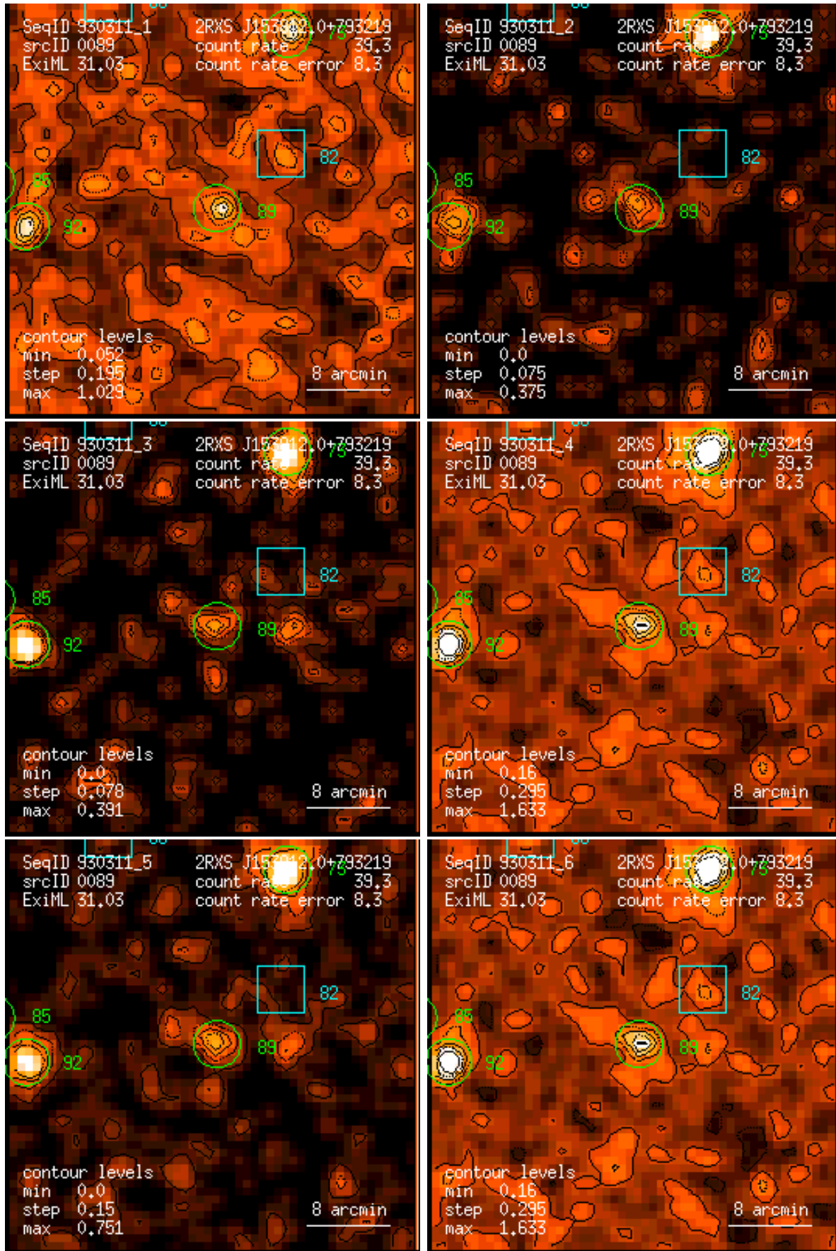
Figure 89: RASS 930311: detection 0089: band rate images, Gaussian filter: (1) PSPC channels 11 – 41, (2) 52 – 90, (3) 91 – 201, (4) 11 – 235, (5) 52 – 201, (6) 11 – 201. Broad band rates in counts/ks. Band rate contour levels in counts/ks/arcmin 2 .
