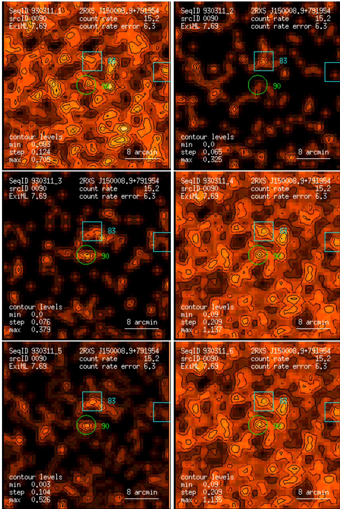
Figure 90: RASS 930311: detection 0090: band rate images, Gaussian filter: (1) PSPC channels 11 – 41, (2) 52 – 90, (3) 91 – 201, (4) 11 – 235, (5) 52 – 201, (6) 11 – 201. Broad band rates in counts/ks. Band rate contour levels in counts/ks/arcmin 2 .
