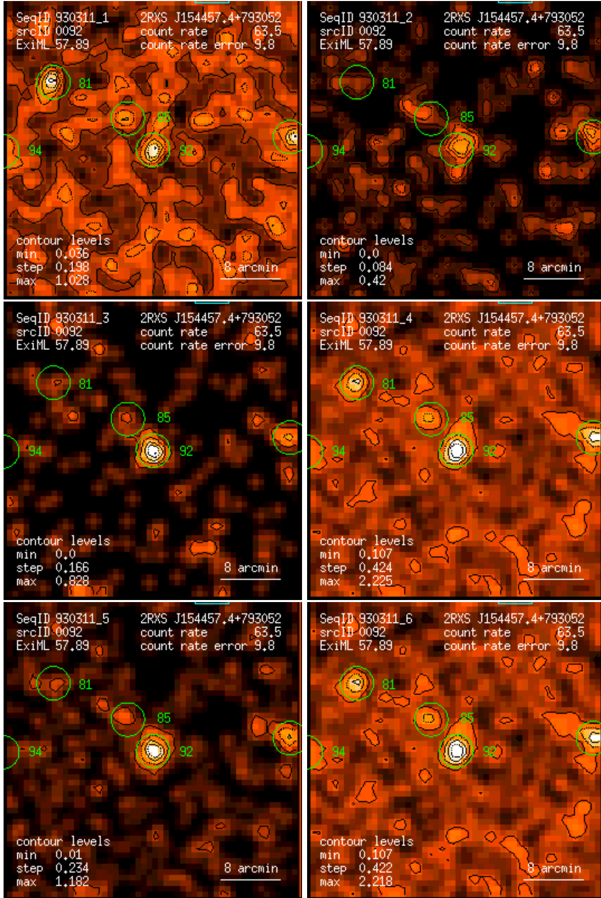
Figure 92: RASS 930311: detection 0092: band rate images, Gaussian filter: (1) PSPC channels 11 – 41, (2) 52 – 90, (3) 91 – 201, (4) 11 – 235, (5) 52 – 201, (6) 11 – 201. Broad band rates in counts/ks. Band rate contour levels in counts/ks/arcmin 2 .
