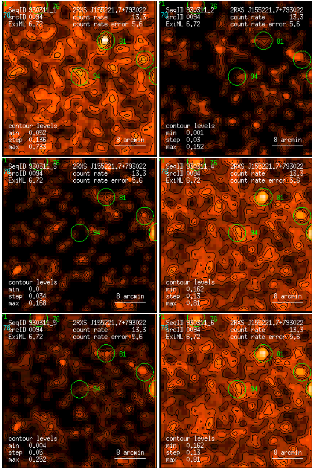
Figure 94: RASS 930311: detection 0094: band rate images, Gaussian filter: (1) PSPC channels 11 – 41, (2) 52 – 90, (3) 91 – 201, (4) 11 – 235, (5) 52 – 201, (6) 11 – 201. Broad band rates in counts/ks. Band rate contour levels in counts/ks/arcmin 2 .
