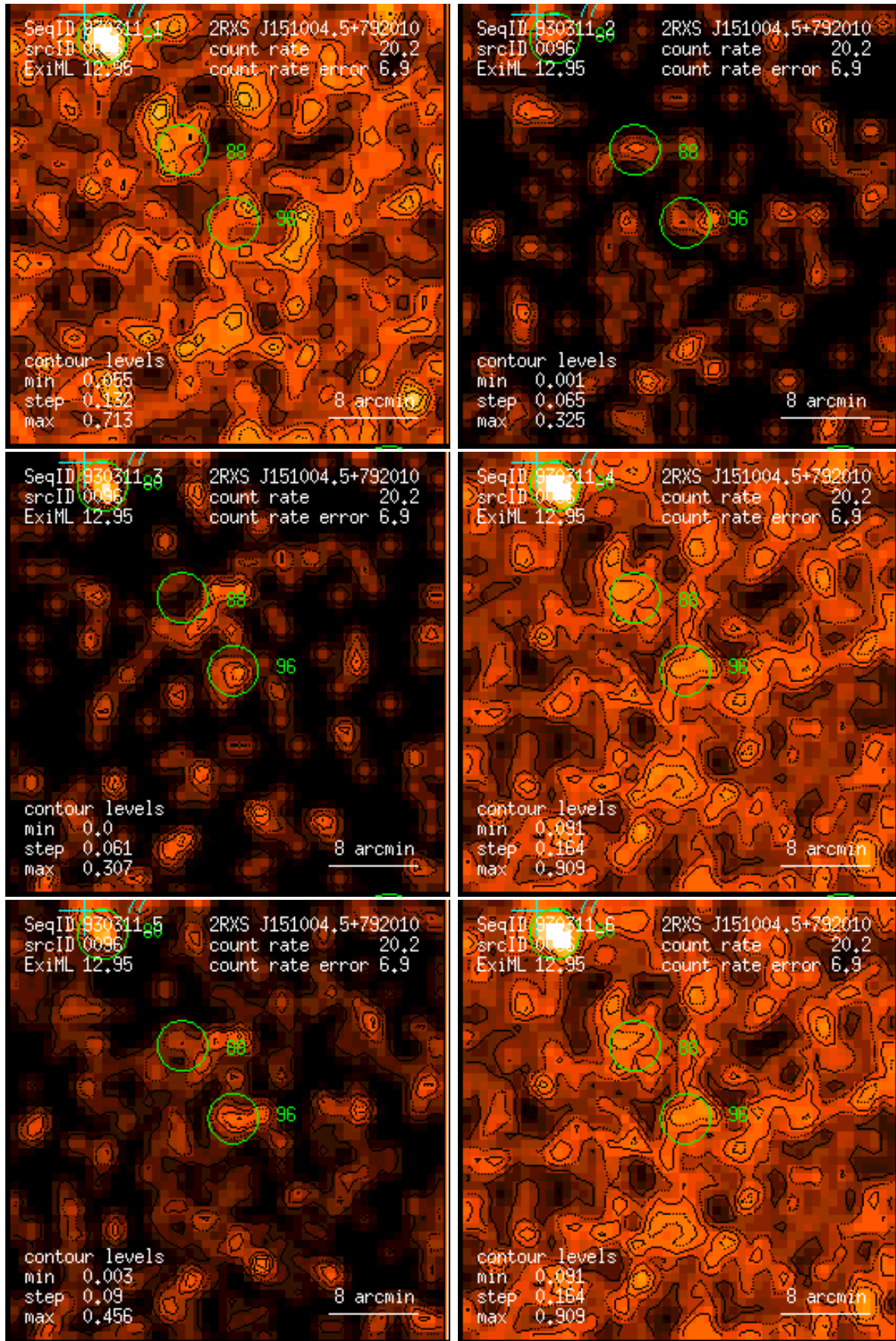
Figure 96: RASS 930311: detection 0096: band rate images, Gaussian filter: (1) PSPC channels 11 – 41, (2) 52 – 90, (3) 91 – 201, (4) 11 – 235, (5) 52 – 201, (6) 11 – 201. Broad band rates in counts/ks. Band rate contour levels in counts/ks/arcmin 2 .
