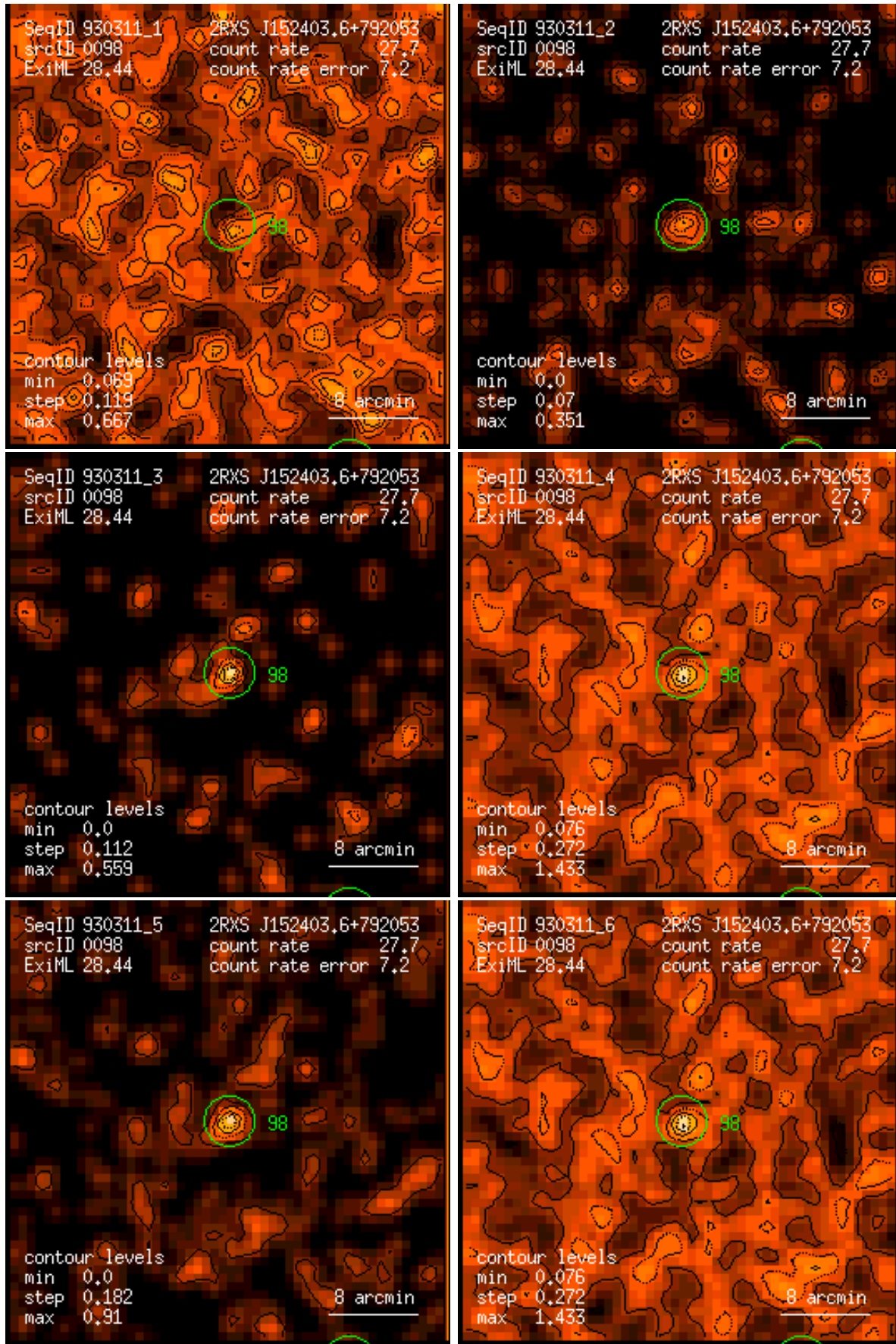
Figure 98: RASS 930311: detection 0098: band rate images, Gaussian filter: (1) PSPC channels 11 – 41, (2) 52 – 90, (3) 91 – 201, (4) 11 – 235, (5) 52 – 201, (6) 11 – 201. Broad band rates in counts/ks. Band rate contour levels in counts/ks/arcmin 2 .
