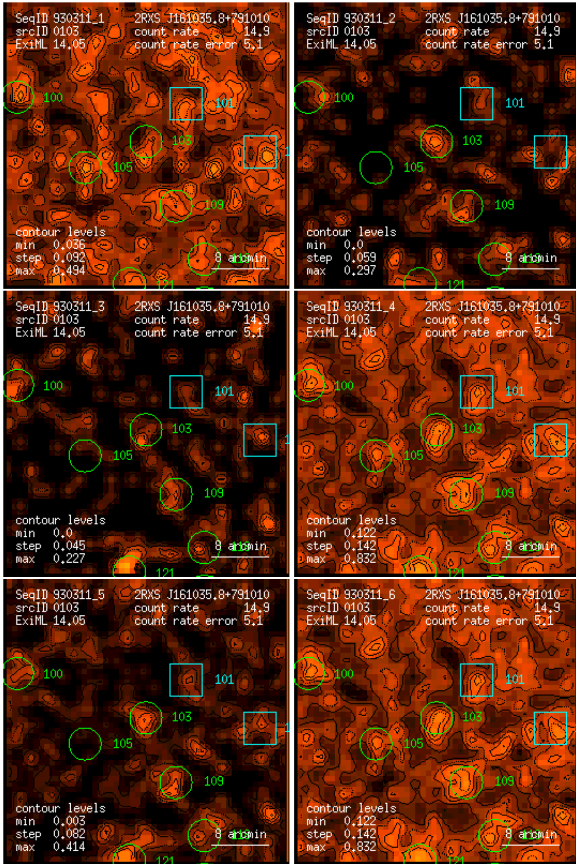
Figure 103: RASS 930311: detection 0103: band rate images, Gaussian filter: (1) PSPC channels 11 – 41, (2) 52 – 90, (3) 91 – 201, (4) 11 – 235, (5) 52 – 201, (6) 11 – 201. Broad band rates in counts/ks. Band rate contour levels in counts/ks/arcmin 2 .
