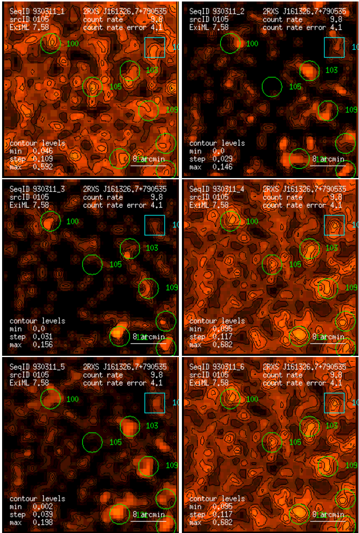
Figure 105: RASS 930311: detection 0105: band rate images, Gaussian filter: (1) PSPC channels 11 – 41, (2) 52 – 90, (3) 91 – 201, (4) 11 – 235, (5) 52 – 201, (6) 11 – 201. Broad band rates in counts/ks. Band rate contour levels in counts/ks/arcmin 2 .
