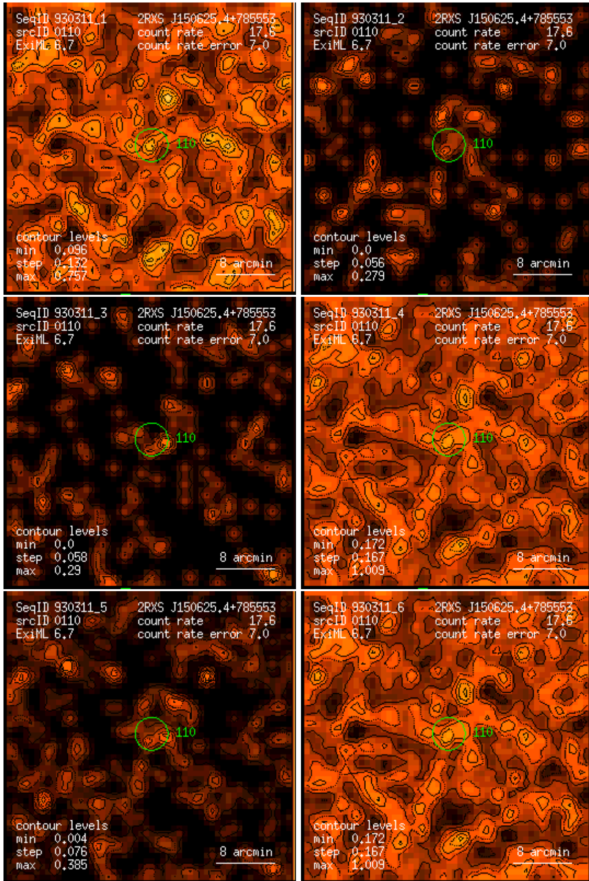
Figure 110: RASS 930311: detection 0110: band rate images, Gaussian filter: (1) PSPC channels 11 – 41, (2) 52 – 90, (3) 91 – 201, (4) 11 – 235, (5) 52 – 201, (6) 11 – 201. Broad band rates in counts/ks. Band rate contour levels in counts/ks/arcmin 2 .
