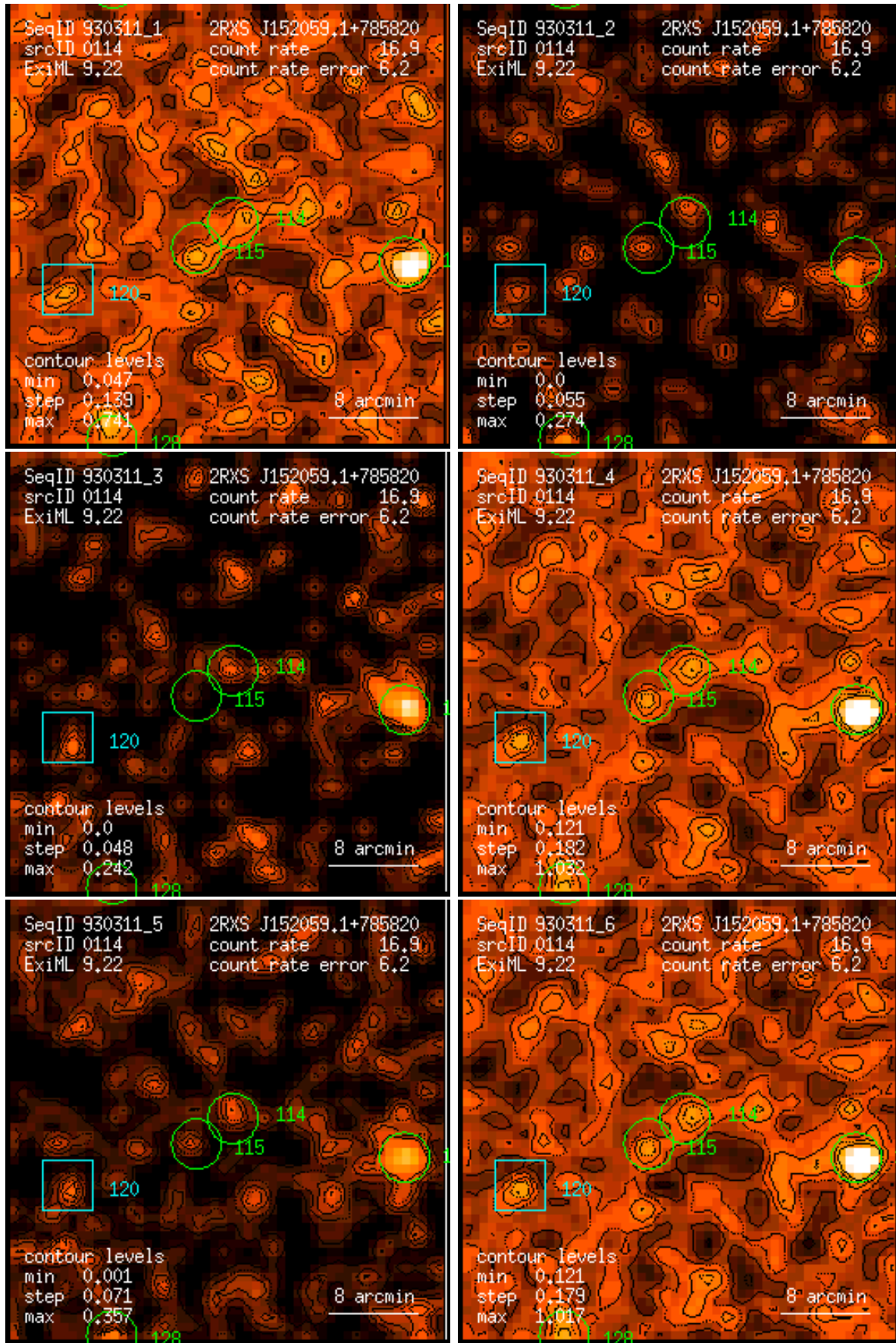
Figure 114: RASS 930311: detection 0114: band rate images, Gaussian filter: (1) PSPC channels 11 – 41, (2) 52 – 90, (3) 91 – 201, (4) 11 – 235, (5) 52 – 201, (6) 11 – 201. Broad band rates in counts/ks. Band rate contour levels in counts/ks/arcmin 2 .
