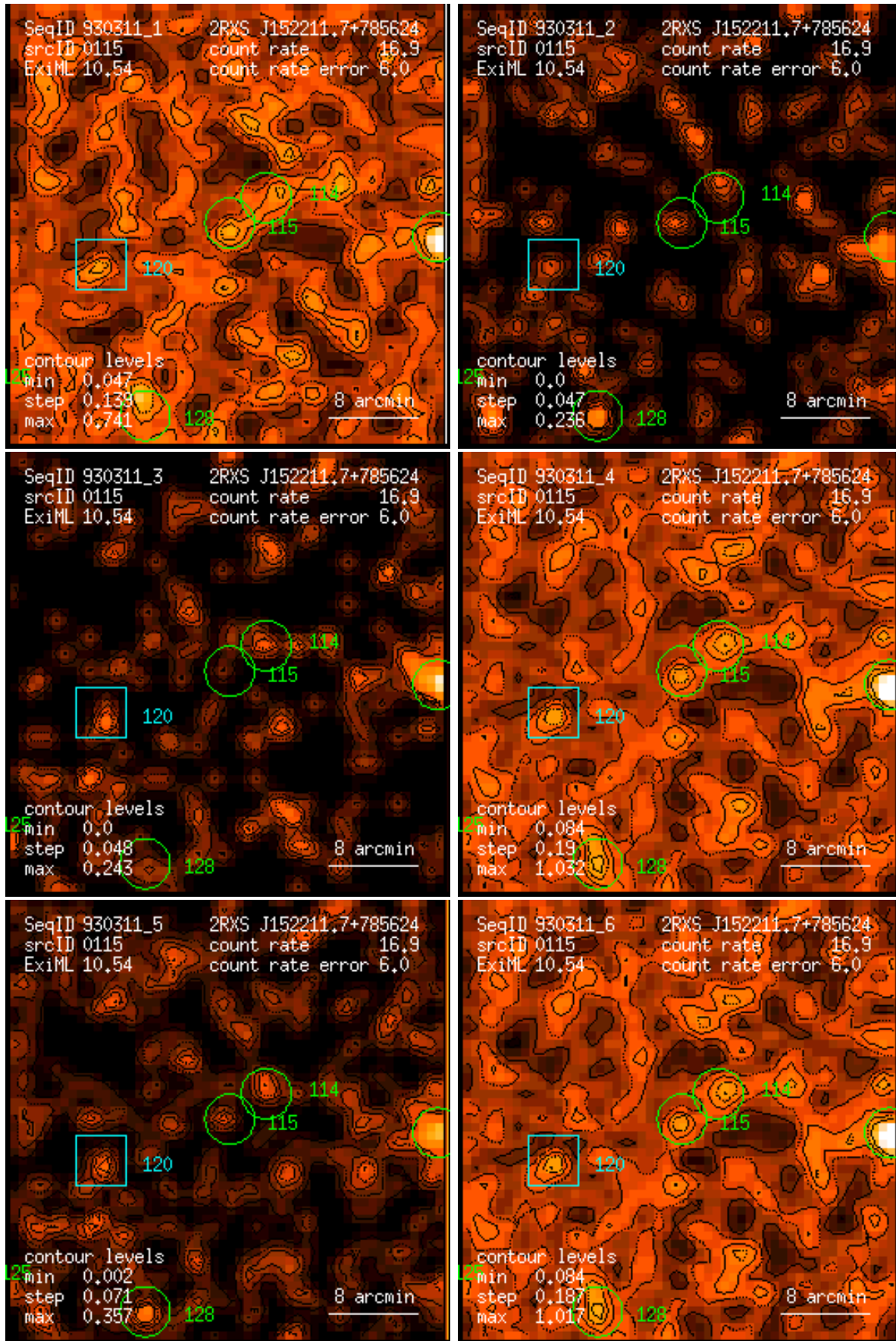
Figure 115: RASS 930311: detection 0115: band rate images, Gaussian filter: (1) PSPC channels 11 – 41, (2) 52 – 90, (3) 91 – 201, (4) 11 – 235, (5) 52 – 201, (6) 11 – 201. Broad band rates in counts/ks. Band rate contour levels in counts/ks/arcmin 2 .
