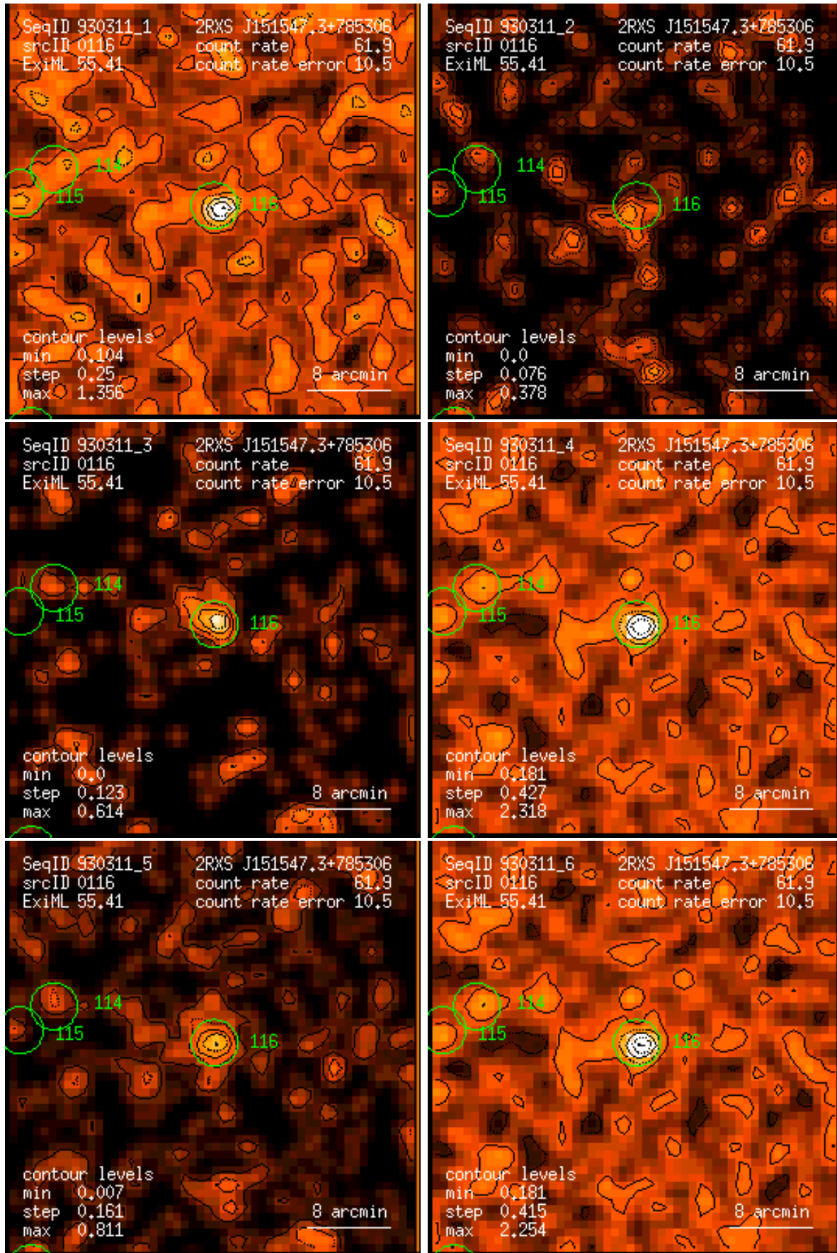
Figure 116: RASS 930311: detection 0116: band rate images, Gaussian filter: (1) PSPC channels 11 – 41, (2) 52 – 90, (3) 91 – 201, (4) 11 – 235, (5) 52 – 201, (6) 11 – 201. Broad band rates in counts/ks. Band rate contour levels in counts/ks/arcmin 2 .
