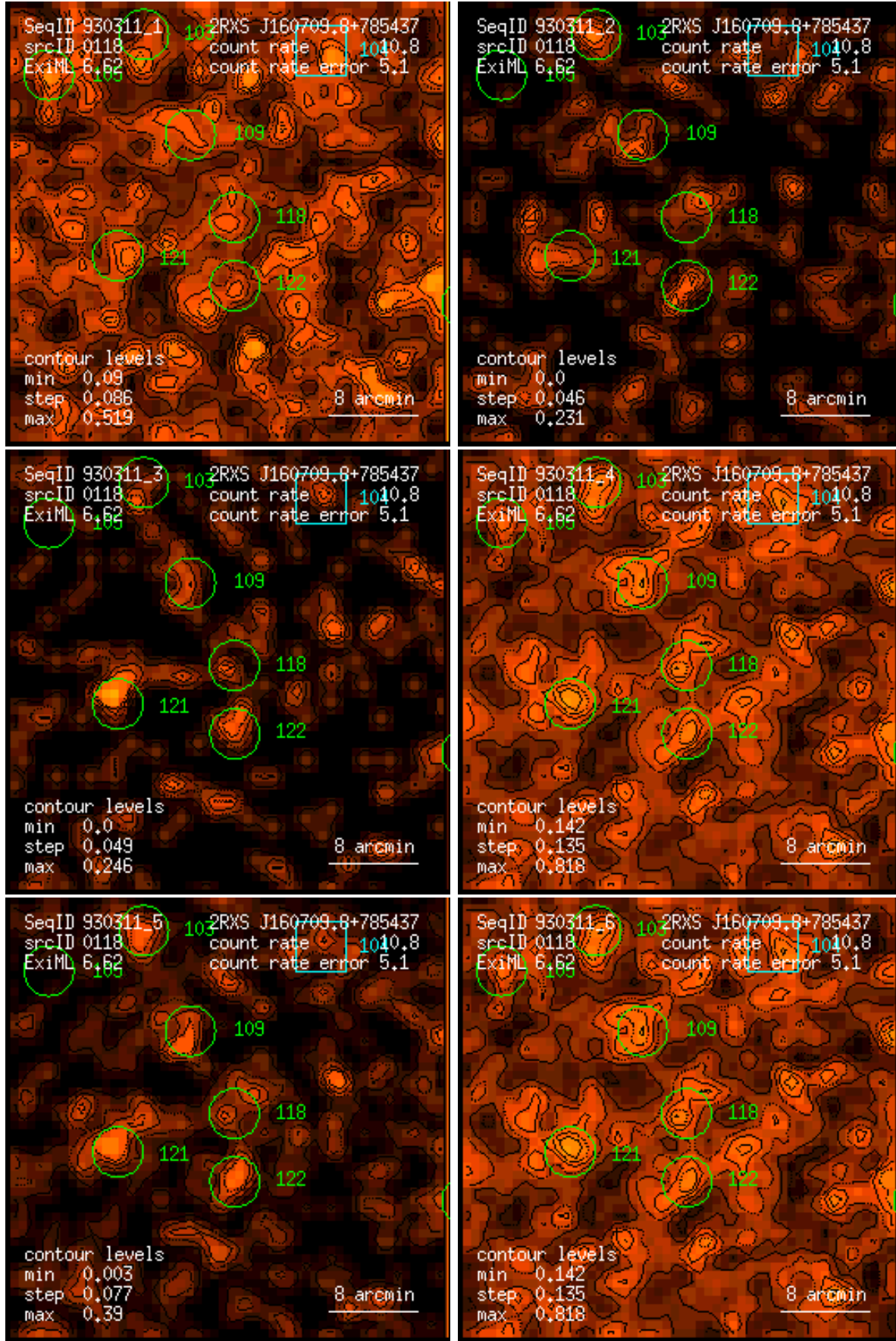
Figure 118: RASS 930311: detection 0118: band rate images, Gaussian filter: (1) PSPC channels 11 – 41, (2) 52 – 90, (3) 91 – 201, (4) 11 – 235, (5) 52 – 201, (6) 11 – 201. Broad band rates in counts/ks. Band rate contour levels in counts/ks/arcmin 2 .
