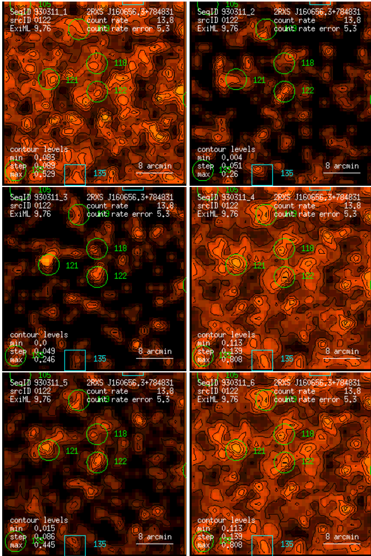
Figure 122: RASS 930311: detection 0122: band rate images, Gaussian filter: (1) PSPC channels 11 – 41, (2) 52 – 90, (3) 91 – 201, (4) 11 – 235, (5) 52 – 201, (6) 11 – 201. Broad band rates in counts/ks. Band rate contour levels in counts/ks/arcmin 2 .
