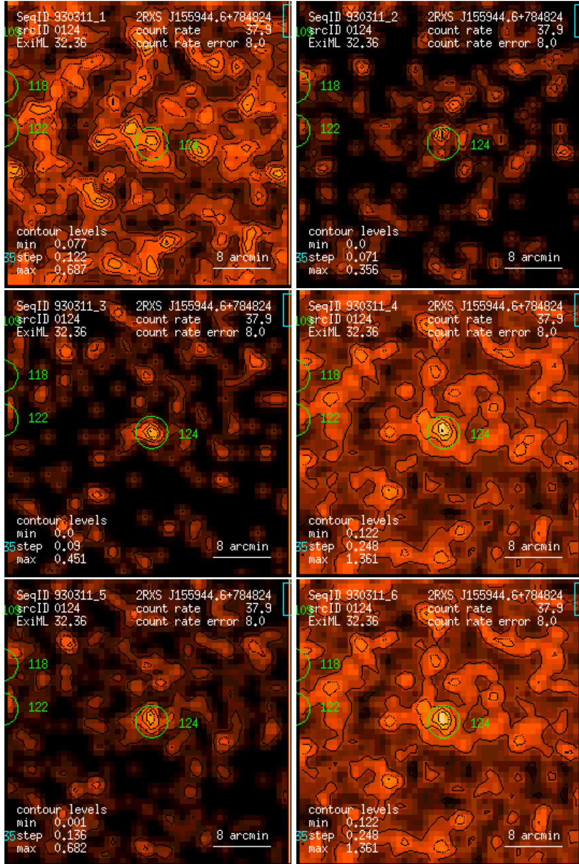
Figure 124: RASS 930311: detection 0124: band rate images, Gaussian filter: (1) PSPC channels 11 – 41, (2) 52 – 90, (3) 91 – 201, (4) 11 – 235, (5) 52 – 201, (6) 11 – 201. Broad band rates in counts/ks. Band rate contour levels in counts/ks/arcmin 2 .
