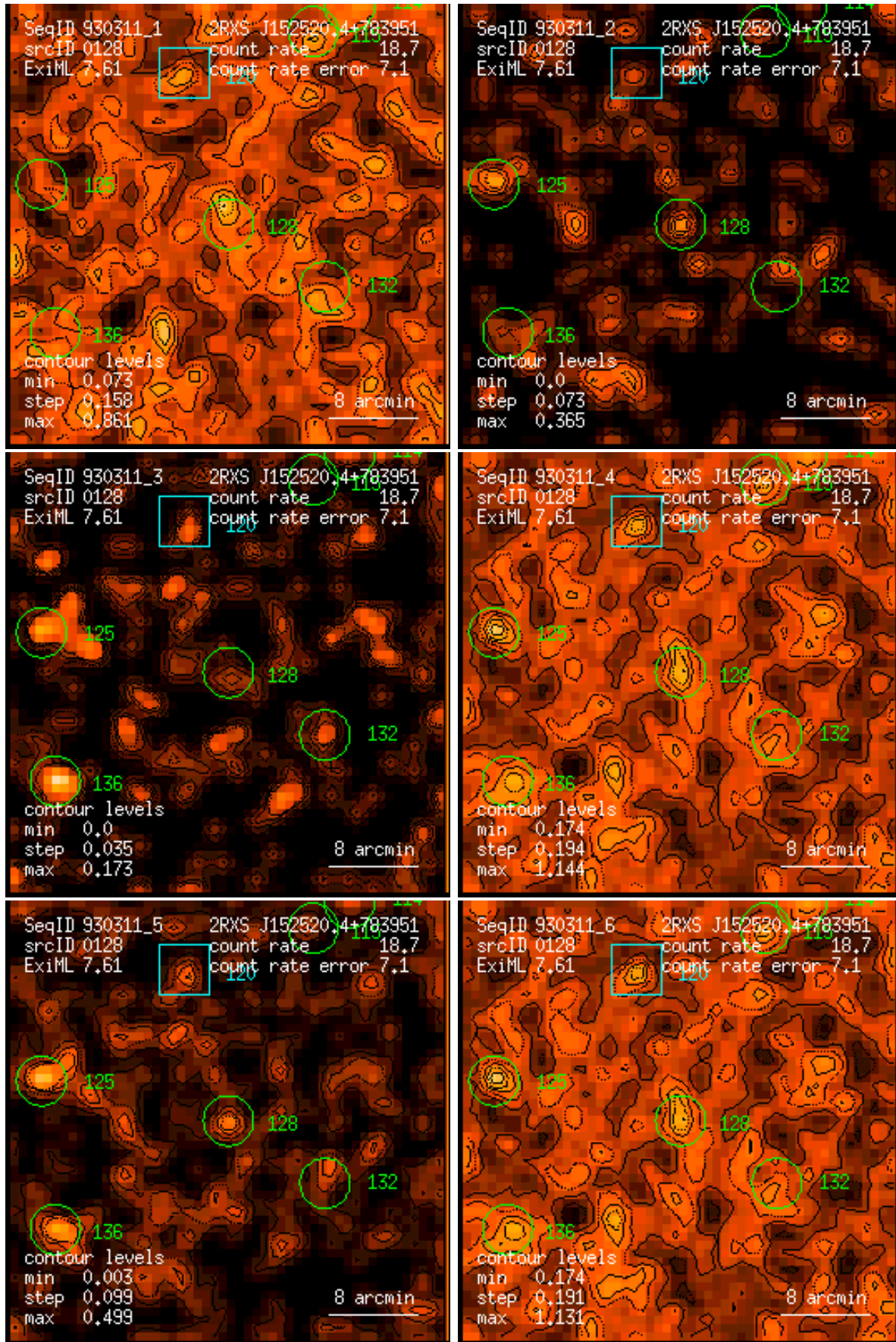
Figure 128: RASS 930311: detection 0128: band rate images, Gaussian filter: (1) PSPC channels 11 – 41, (2) 52 – 90, (3) 91 – 201, (4) 11 – 235, (5) 52 – 201, (6) 11 – 201. Broad band rates in counts/ks. Band rate contour levels in counts/ks/arcmin 2 .
