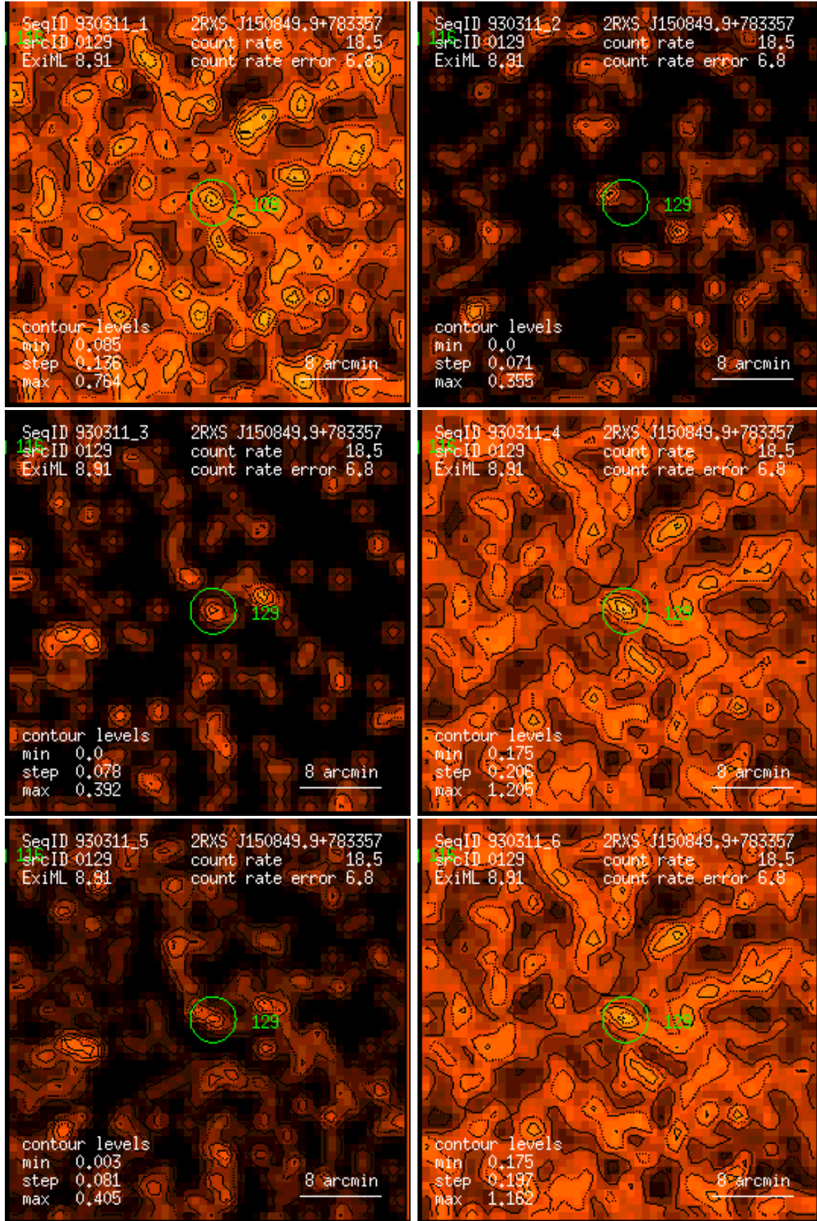
Figure 129: RASS 930311: detection 0129: band rate images, Gaussian filter: (1) PSPC channels 11 – 41, (2) 52 – 90, (3) 91 – 201, (4) 11 – 235, (5) 52 – 201, (6) 11 – 201. Broad band rates in counts/ks. Band rate contour levels in counts/ks/arcmin 2 .
