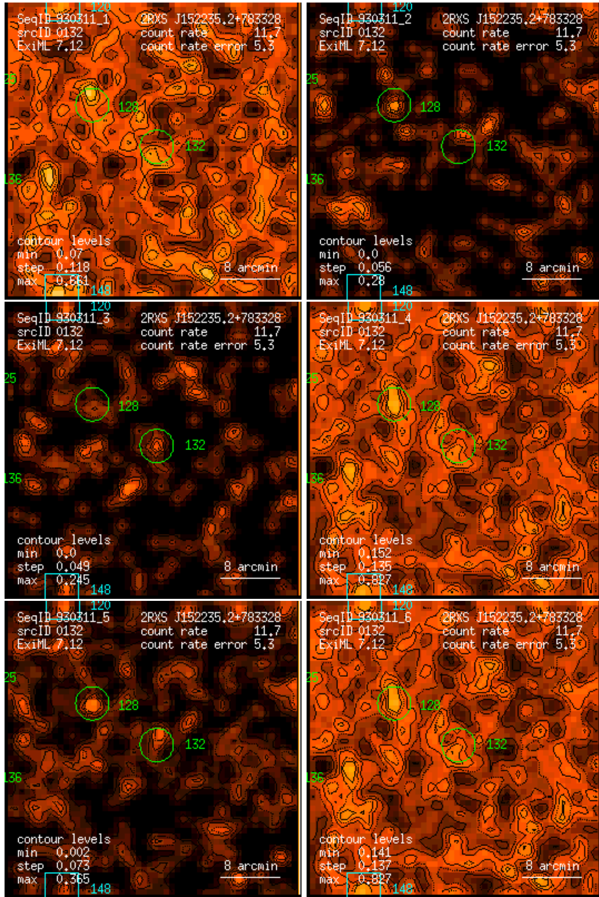
Figure 132: RASS 930311: detection 0132: band rate images, Gaussian filter: (1) PSPC channels 11 – 41, (2) 52 – 90, (3) 91 – 201, (4) 11 – 235, (5) 52 – 201, (6) 11 – 201. Broad band rates in counts/ks. Band rate contour levels in counts/ks/arcmin 2 .
