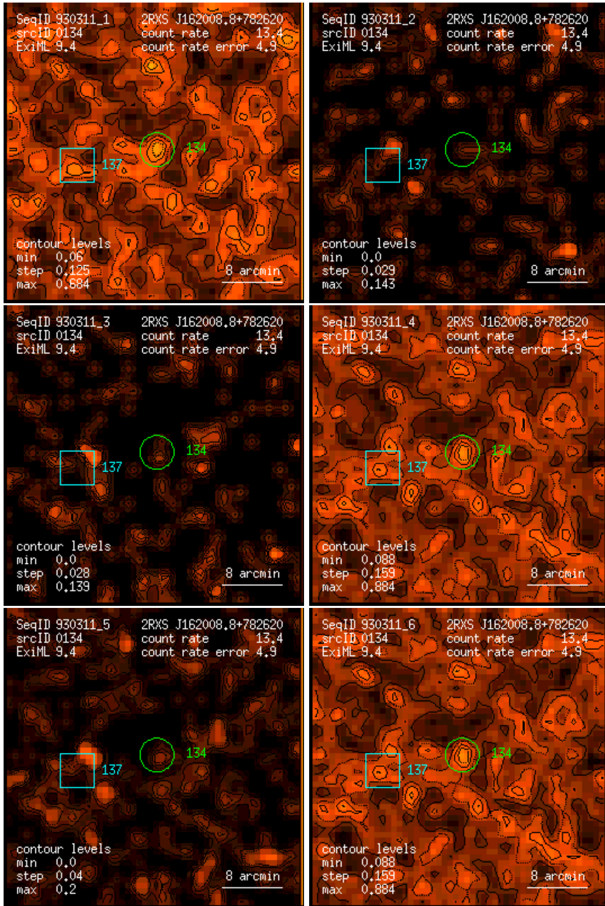
Figure 134: RASS 930311: detection 0134: band rate images, Gaussian filter: (1) PSPC channels 11 – 41, (2) 52 – 90, (3) 91 – 201, (4) 11 – 235, (5) 52 – 201, (6) 11 – 201. Broad band rates in counts/ks. Band rate contour levels in counts/ks/arcmin 2 .
