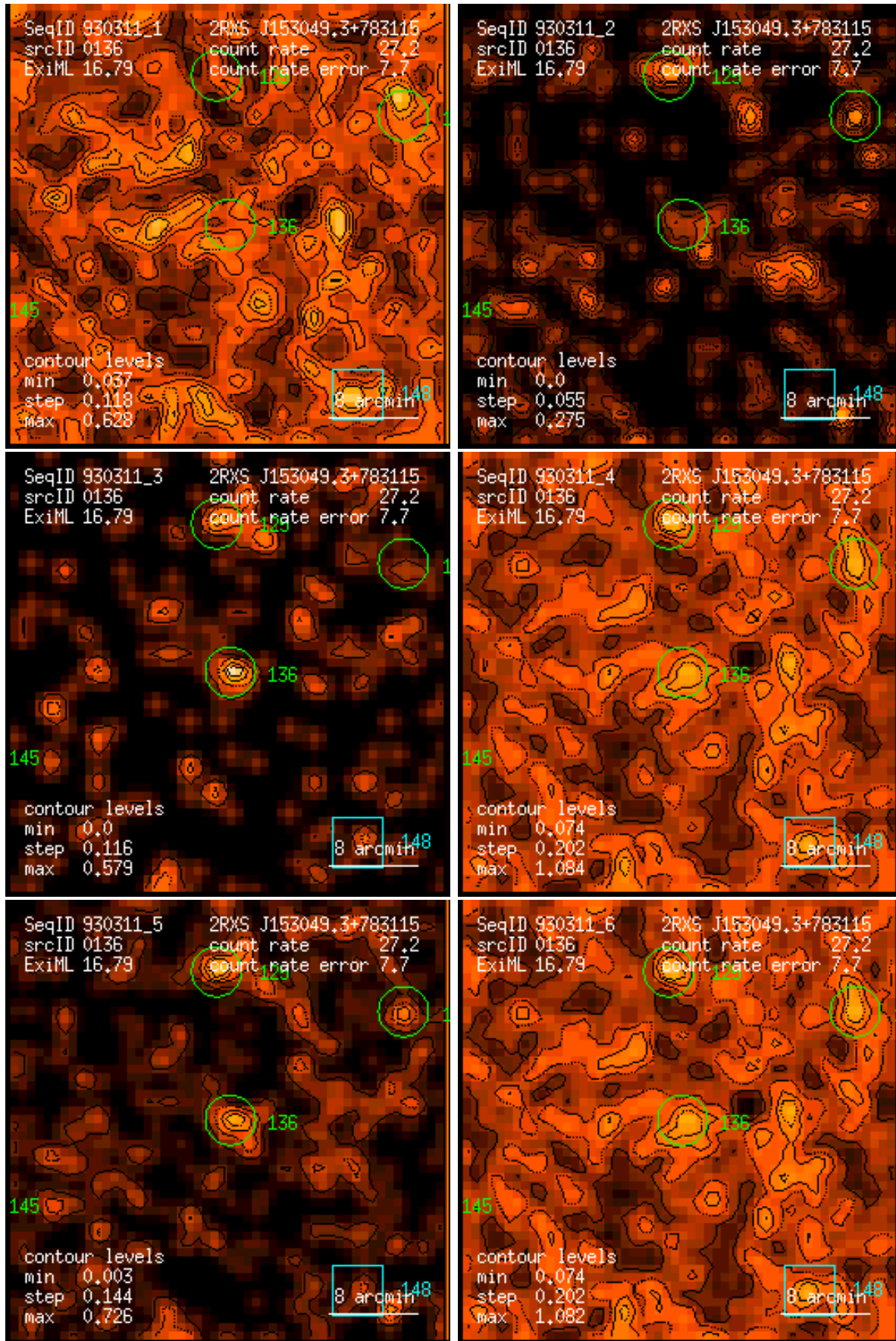
Figure 136: RASS 930311: detection 0136: band rate images, Gaussian filter: (1) PSPC channels 11 – 41, (2) 52 – 90, (3) 91 – 201, (4) 11 – 235, (5) 52 – 201, (6) 11 – 201. Broad band rates in counts/ks. Band rate contour levels in counts/ks/arcmin 2 .
