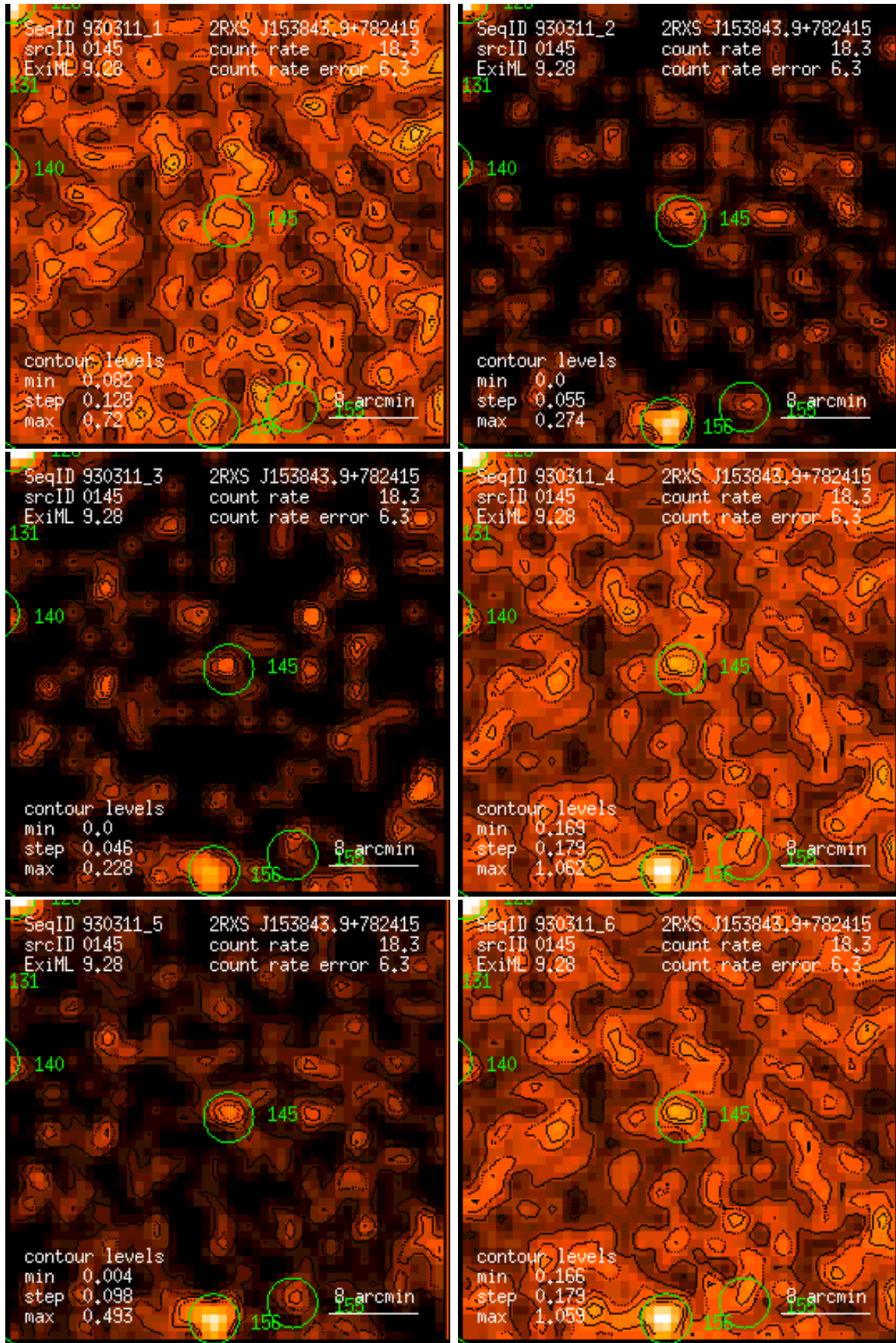
Figure 145: RASS 930311: detection 0145: band rate images, Gaussian filter: (1) PSPC channels 11 – 41, (2) 52 – 90, (3) 91 – 201, (4) 11 – 235, (5) 52 – 201, (6) 11 – 201. Broad band rates in counts/ks. Band rate contour levels in counts/ks/arcmin 2 .
