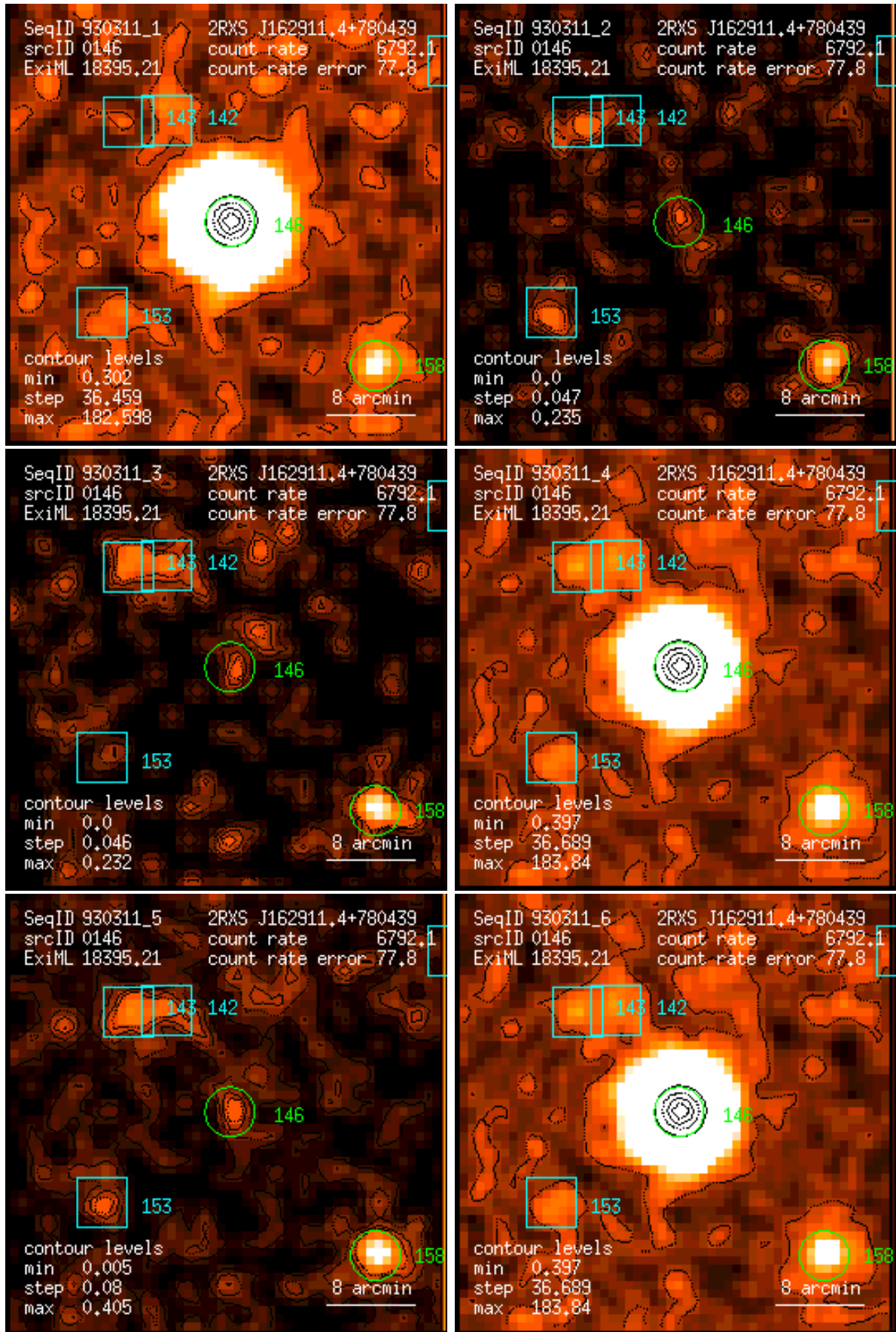
Figure 146: RASS 930311: detection 0146: band rate images, Gaussian filter: (1) PSPC channels 11 – 41, (2) 52 – 90, (3) 91 – 201, (4) 11 – 235, (5) 52 – 201, (6) 11 – 201. Broad band rates in counts/ks. Band rate contour levels in counts/ks/arcmin 2 .
