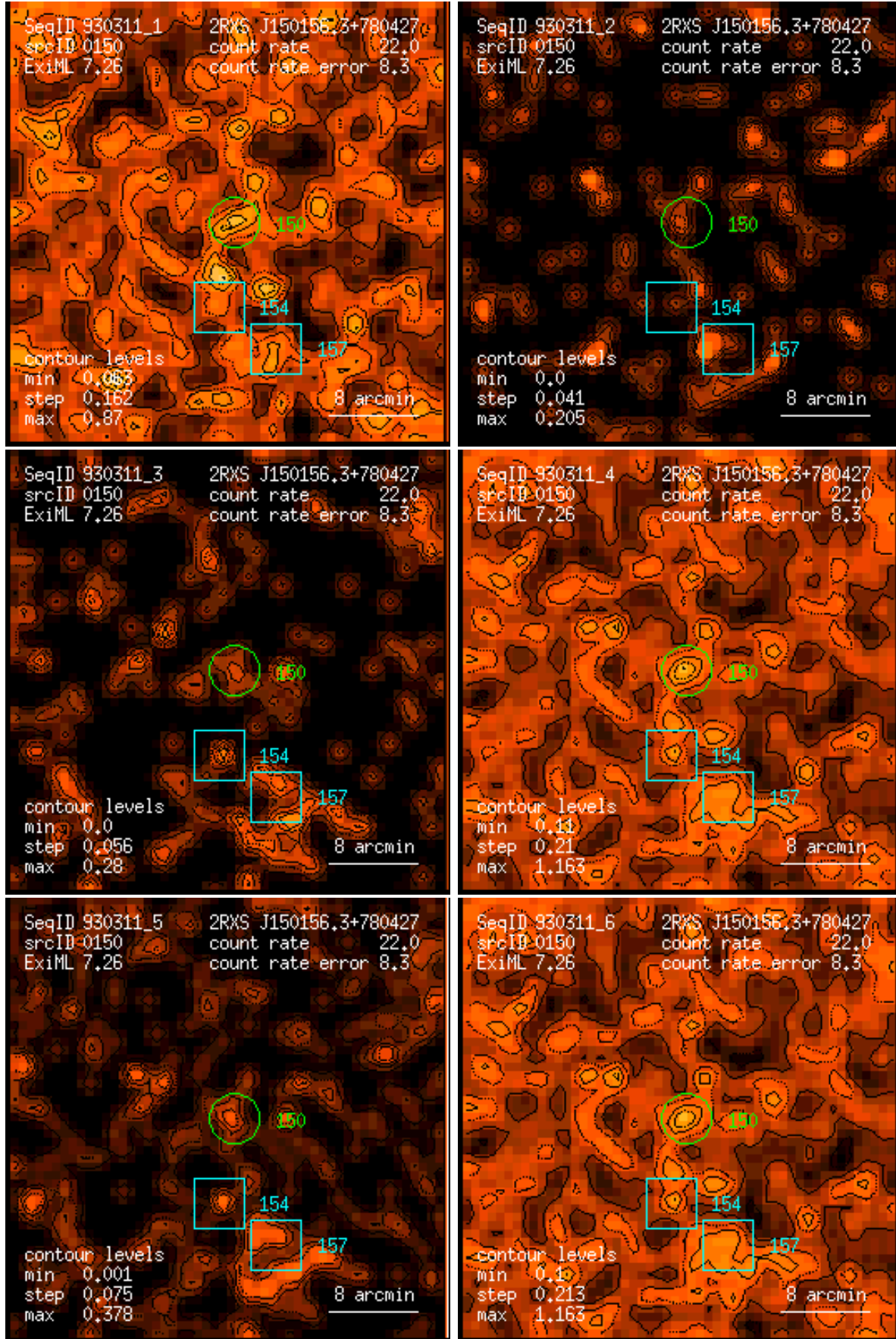
Figure 150: RASS 930311: detection 0150: band rate images, Gaussian filter: (1) PSPC channels 11 – 41, (2) 52 – 90, (3) 91 – 201, (4) 11 – 235, (5) 52 – 201, (6) 11 – 201. Broad band rates in counts/ks. Band rate contour levels in counts/ks/arcmin 2 .
