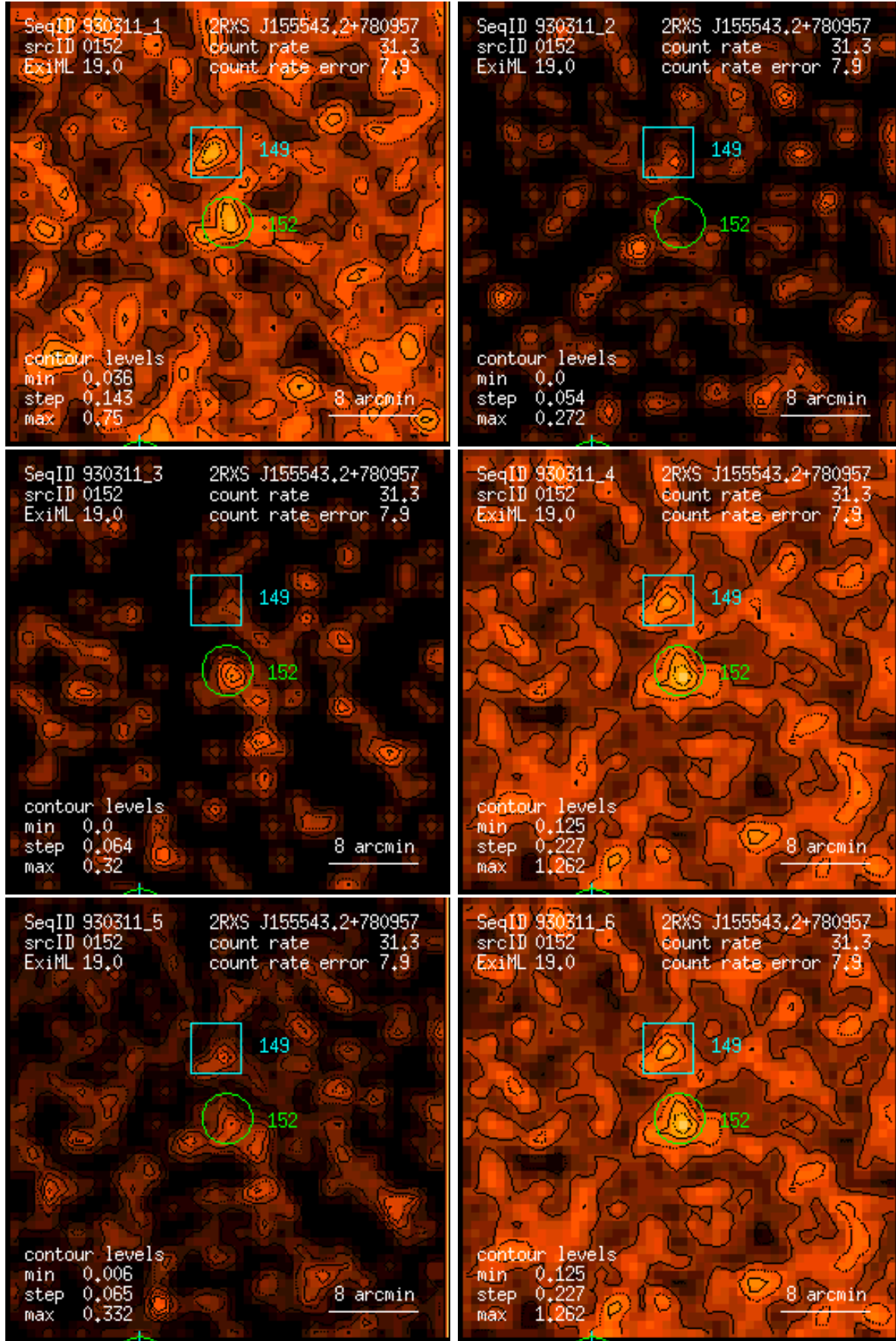
Figure 152: RASS 930311: detection 0152: band rate images, Gaussian filter: (1) PSPC channels 11 – 41, (2) 52 – 90, (3) 91 – 201, (4) 11 – 235, (5) 52 – 201, (6) 11 – 201. Broad band rates in counts/ks. Band rate contour levels in counts/ks/arcmin 2 .
