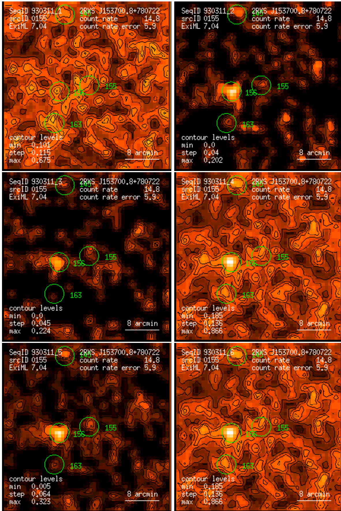
Figure 155: RASS 930311: detection 0155: band rate images, Gaussian filter: (1) PSPC channels 11 – 41, (2) 52 – 90, (3) 91 – 201, (4) 11 – 235, (5) 52 – 201, (6) 11 – 201. Broad band rates in counts/ks. Band rate contour levels in counts/ks/arcmin 2 .
