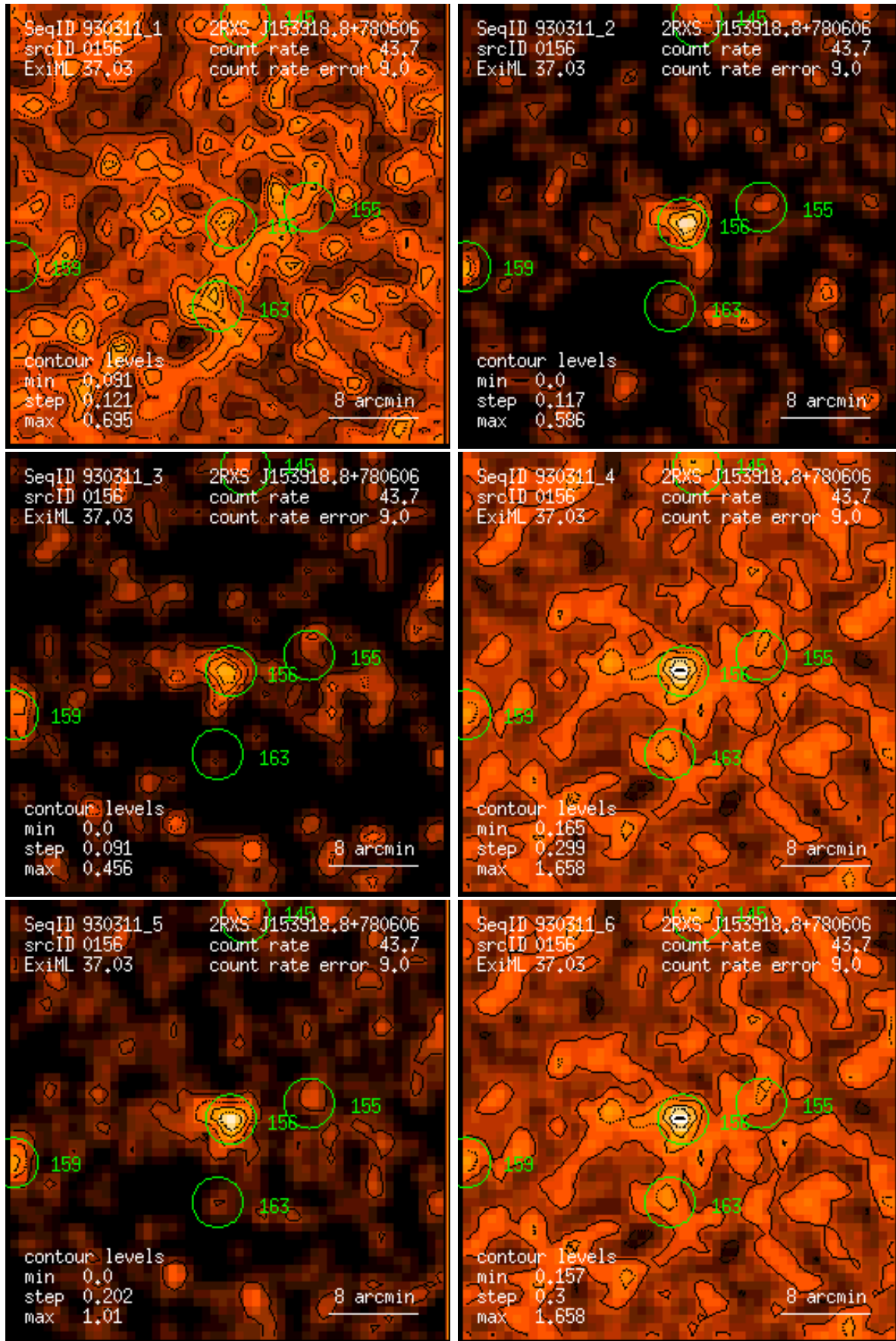
Figure 156: RASS 930311: detection 0156: band rate images, Gaussian filter: (1) PSPC channels 11 – 41, (2) 52 – 90, (3) 91 – 201, (4) 11 – 235, (5) 52 – 201, (6) 11 – 201. Broad band rates in counts/ks. Band rate contour levels in counts/ks/arcmin 2 .
