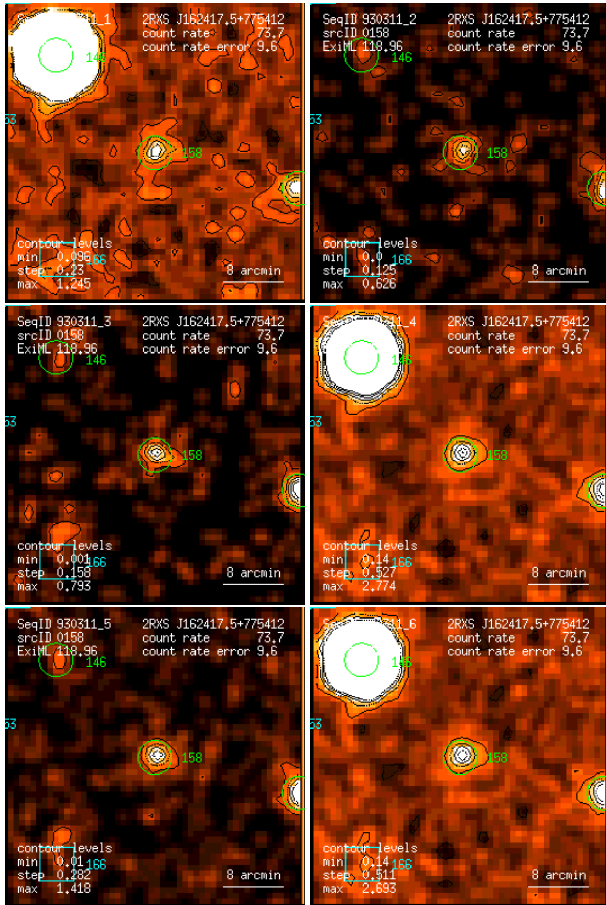
Figure 158: RASS 930311: detection 0158: band rate images, Gaussian filter: (1) PSPC channels 11 – 41, (2) 52 – 90, (3) 91 – 201, (4) 11 – 235, (5) 52 – 201, (6) 11 – 201. Broad band rates in counts/ks. Band rate contour levels in counts/ks/arcmin 2 .
