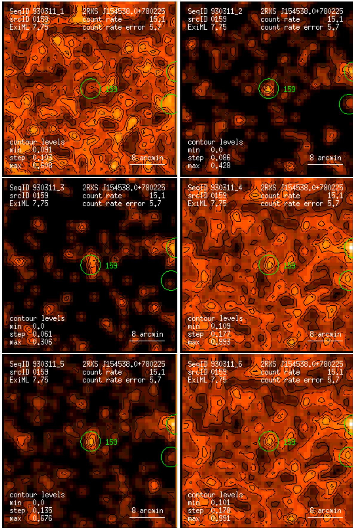
Figure 159: RASS 930311: detection 0159: band rate images, Gaussian filter: (1) PSPC channels 11 – 41, (2) 52 – 90, (3) 91 – 201, (4) 11 – 235, (5) 52 – 201, (6) 11 – 201. Broad band rates in counts/ks. Band rate contour levels in counts/ks/arcmin 2 .
