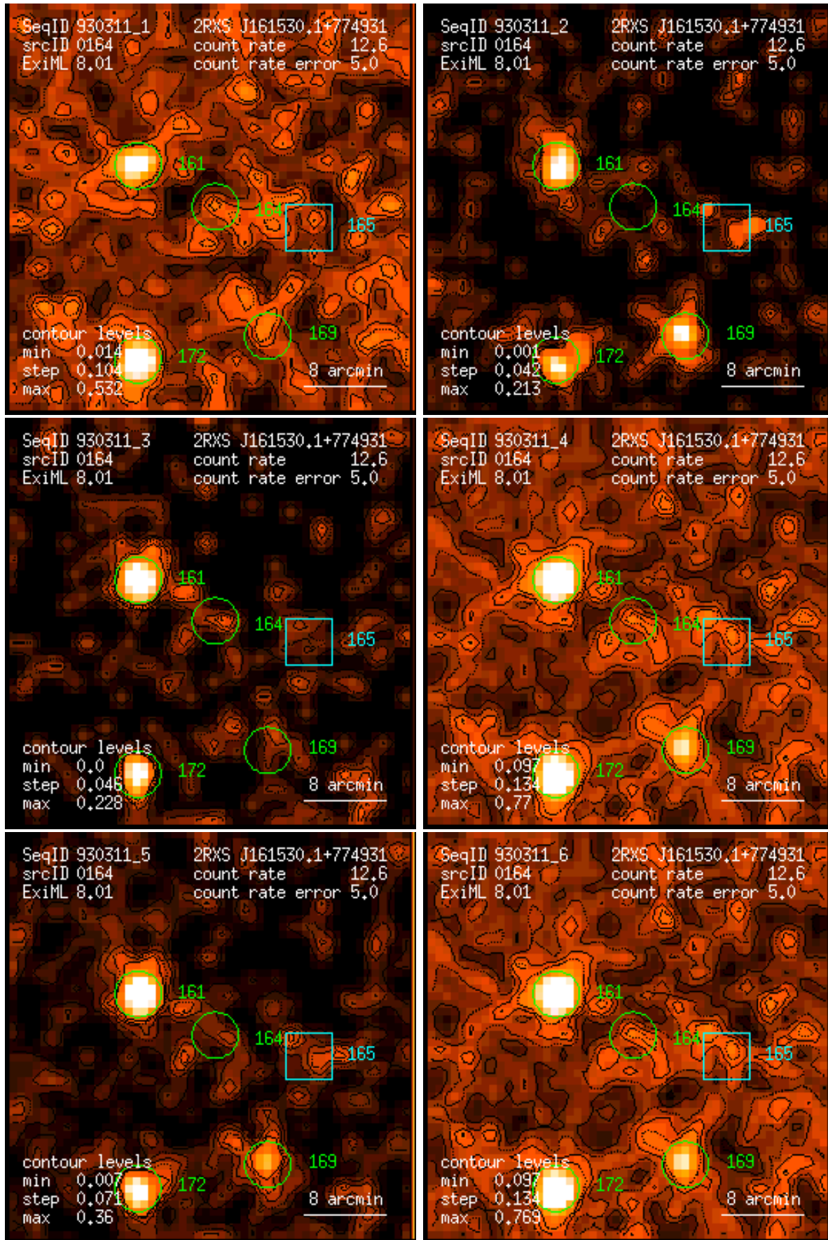
Figure 164: RASS 930311: detection 0164: band rate images, Gaussian filter: (1) PSPC channels 11 – 41, (2) 52 – 90, (3) 91 – 201, (4) 11 – 235, (5) 52 – 201, (6) 11 – 201. Broad band rates in counts/ks. Band rate contour levels in counts/ks/arcmin 2 .
