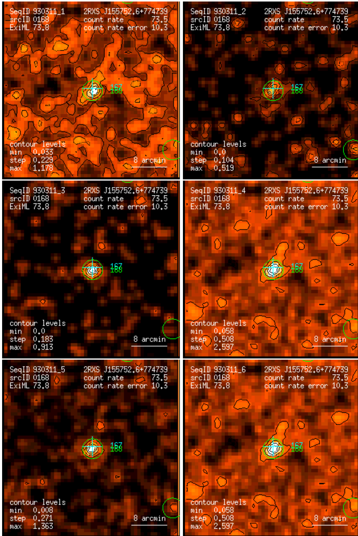
Figure 168: RASS 930311: detection 0168: band rate images, Gaussian filter: (1) PSPC channels 11 – 41, (2) 52 – 90, (3) 91 – 201, (4) 11 – 235, (5) 52 – 201, (6) 11 – 201. Broad band rates in counts/ks. Band rate contour levels in counts/ks/arcmin 2 .
