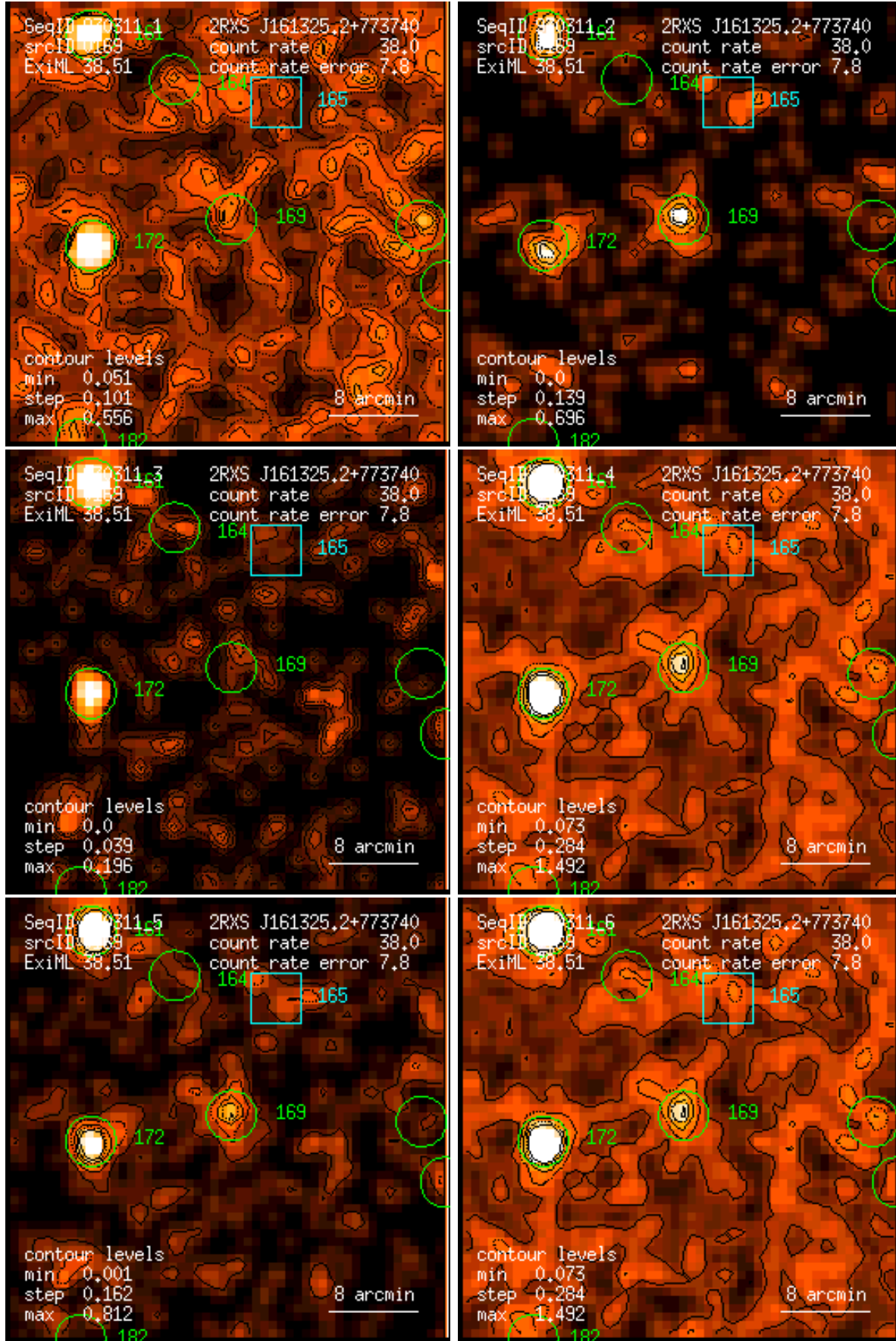
Figure 169: RASS 930311: detection 0169: band rate images, Gaussian filter: (1) PSPC channels 11 – 41, (2) 52 – 90, (3) 91 – 201, (4) 11 – 235, (5) 52 – 201, (6) 11 – 201. Broad band rates in counts/ks. Band rate contour levels in counts/ks/arcmin 2 .
